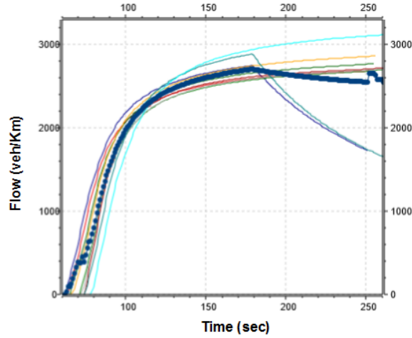
Fig. 9: Average Flow in case of No-Accident with Rogue Nodes
