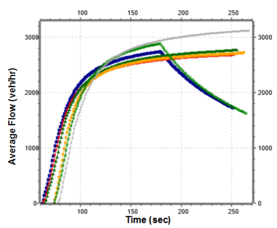
(c) 2 rogue nodes reporting lower values of flow
