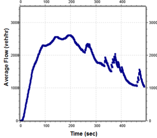
(c) Decreasing flow in case of real accident
