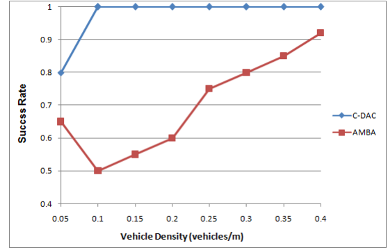
Fig. 8: Percentage of vehicles within the distance 3000m that received the emergency information successfully
