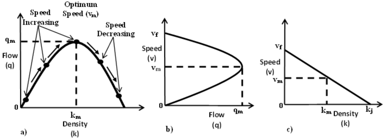
Fig. 1: Greenshield's Fundamental Diagrams (a)Flow vs Density, (b)Speed vs Flow, (c)Speed vs Density
