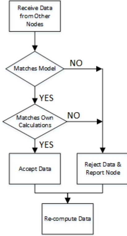
Fig. 3: Overview of Detection And Correction scheme (C-DAC)
