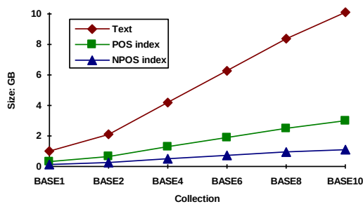
Fig 22a. BASE1-BASE10 local build [ DocId ]: index space costs in Gigabytes
