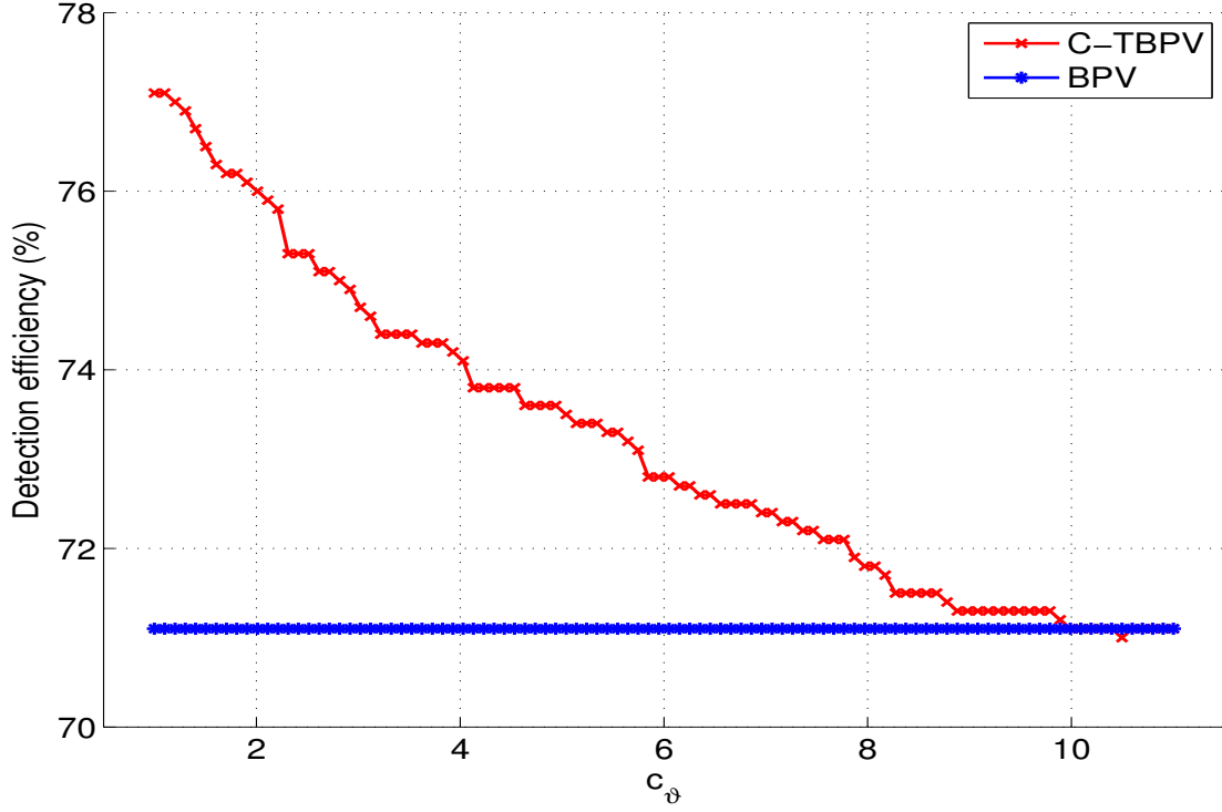
Figure 2: Jump detection power for the model (4.1) in the presence of a single jump, as a function of the threshold parameter c_\theta .
