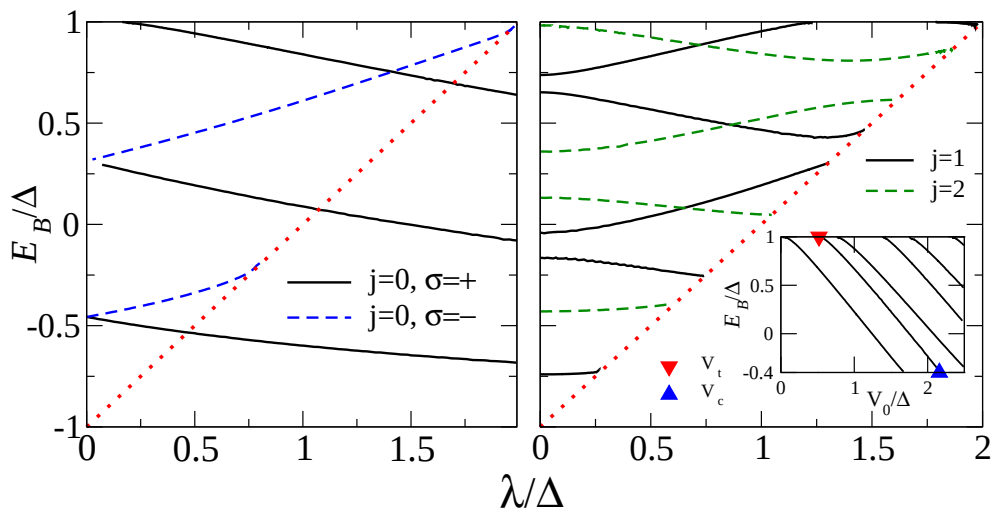
Figure 1. Bound-state spectrum ( E_B ) vs. Rashba SOI ( \lambda ) for a circular potential well with depth V_0 = 2\Delta and radius R = 3/\Delta . Only the lowest-energy states with j = 0, 1, 2 are shown. The red dotted line indicates E_+ = -\Delta + \lambda . The left panel shows j = 0 bound states with parity \sigma = \pm . The right panel shows j = 1, 2 bound states. The inset displays the j = 1 bound-state energies vs. potential depth V_0 for \lambda = 0.6\Delta . At some threshold value V_0 = V_t (where V_t = 0 for the lowest state shown), a new bound state emerges from the conduction band. This state dives into the valence band for some critical value V_0 = V_c > V_t , where the valence band edge is at energy E_B = E_+ = -0.4\Delta . For the second bound state in the inset, V_t ( V_c ) is shown as red (blue) triangle.
