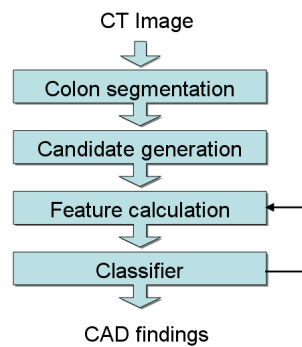
Figure 1. Block diagram for CAD system overview.
