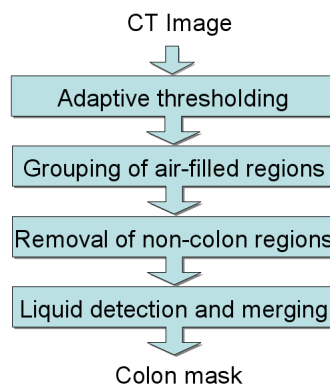
Figure 2. Block diagram for the colon segmentation.
