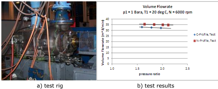
Figure 4 Oil free compressor HS204/165/260
