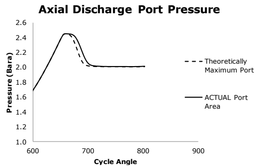
Figure 6 - Pressure history during the discharge process
