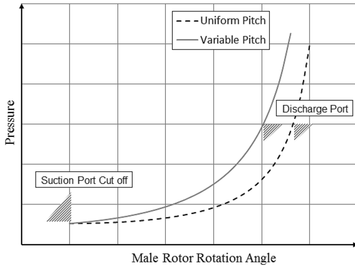
Fig. 5. Pressure-Angle Diagram
