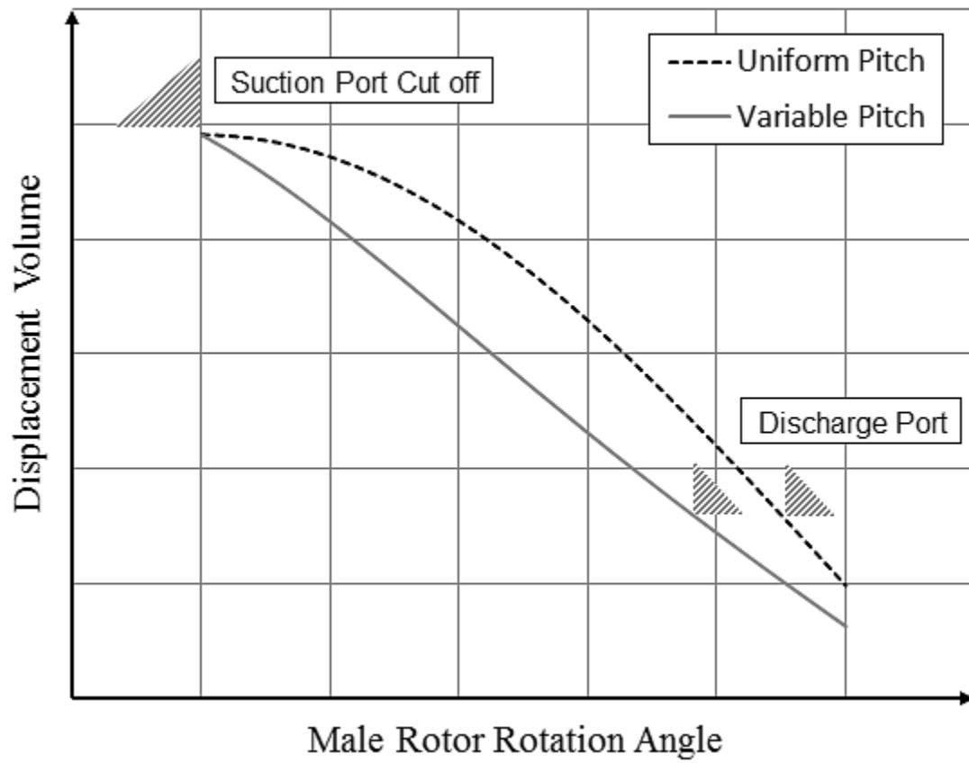
Fig. 4. Volume-Angle diagram
