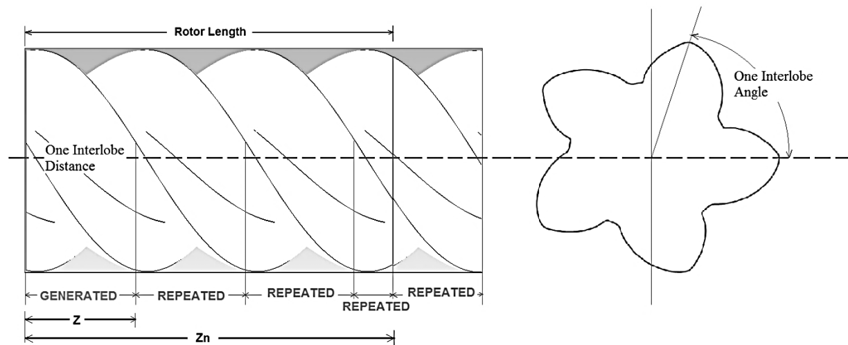
Fig. 9. Uniform Pitch Grid Generation
