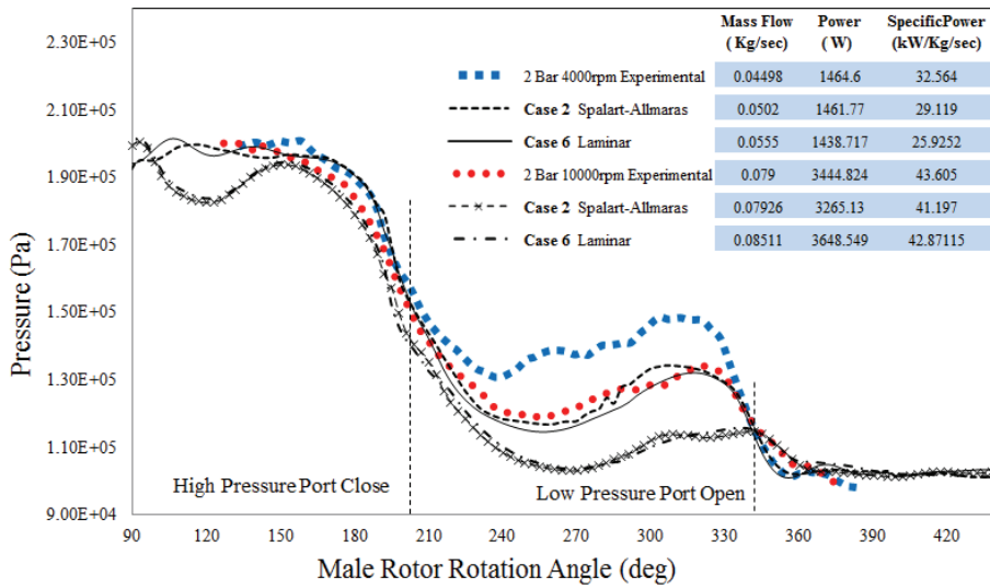
Figure 8. Influence of Laminar and Turbulence model on P-Alfa
