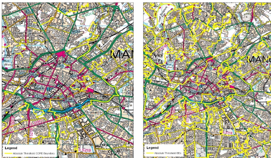
Figure 3. Absolute BLV threshold showing the core and fuzzy Wombed boundaries (in yellow) on a
