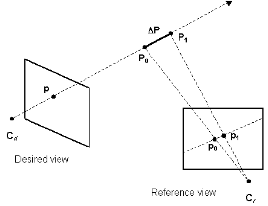
Figure 8: Stepping along an epipolar line.
