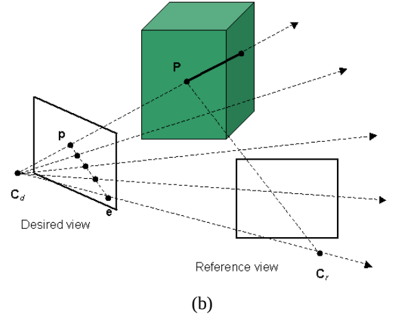
Figure 5: P is visible in the reference view if there is no occluding geometry along \overline{PC_r} .
