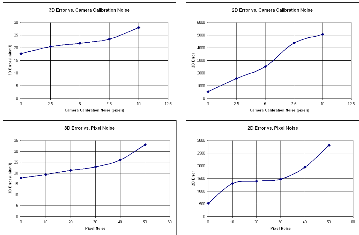
Figure 19: Noise analysis. The upper plots present the 3D and 2D errors as a function of increasing noise in the camera calibration, while the lower plots present the 3D and 2D error as a function of increasing noise added to the image pixels.
