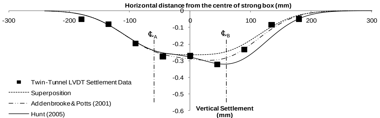
Figure 3 Twin-tunnel settlements
