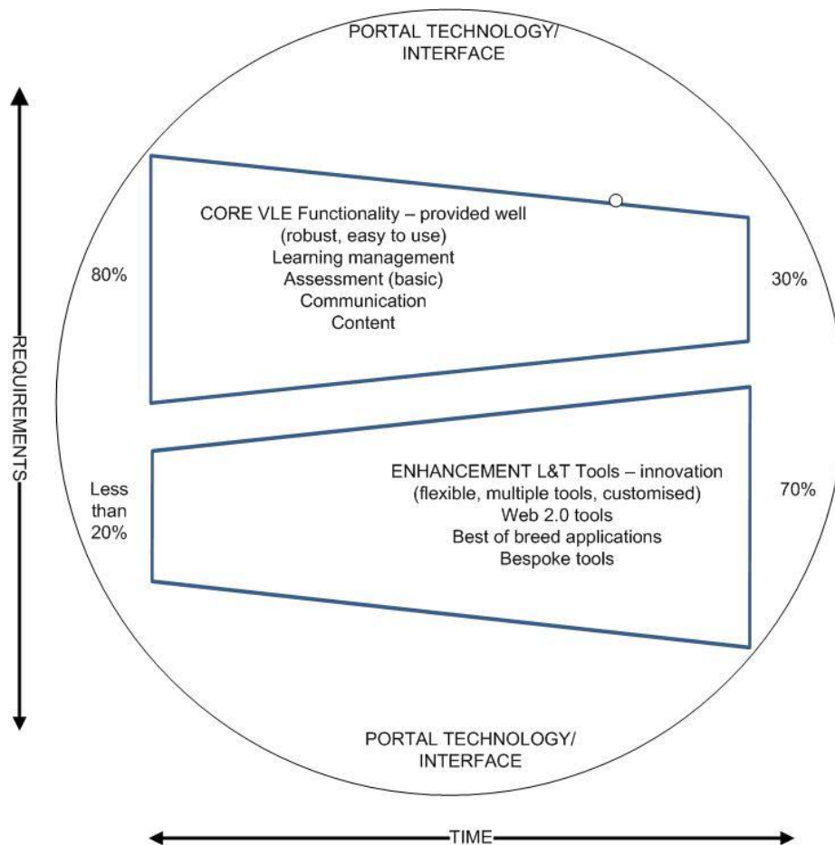
Figure 1: SLE vision
