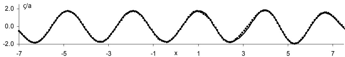
(a) \tau = 10T
