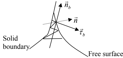
Fig. 6 Nodes near a solid boundary
