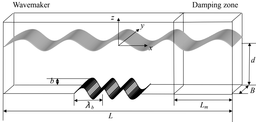
Fig. 1 Sketch of fluid domain
