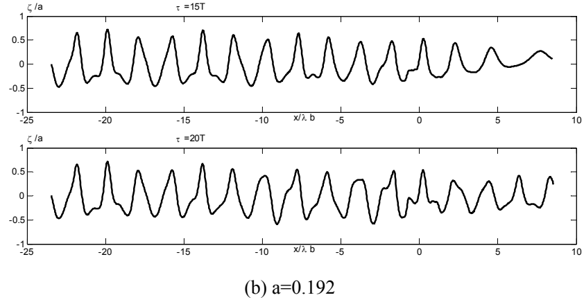
(b) a=0.192 Fig. 16 Wave profiles corresponding to different amplitudes for 4 bars
