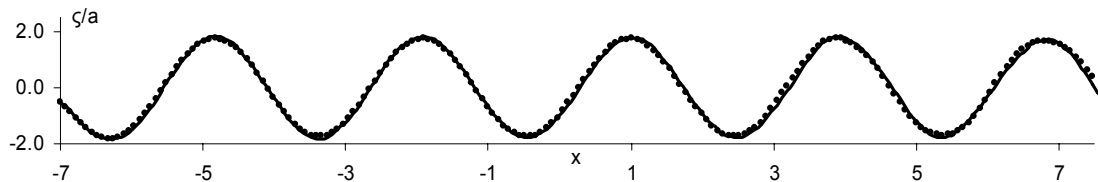
(b) \tau = 15T
