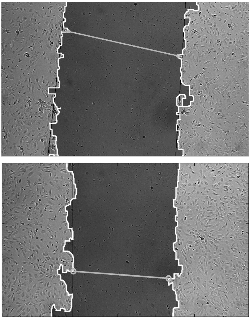
Labelled scratch wound assay at times t = 0, 6, h . The boundaries between cellular regions and the wound are labelled with thick white lines. A thick grey line with circular markers lines represents the shortest distance between boundaries, two thin black lines represent a straight-line approximation of the boundaries, and the intensity of the pixels corresponding to the wound has been darkened. Distances: minimum = 578.7, 495.2, average = 624, 538, pixels, relative area of the wound = 49.9, 43.2, %.
