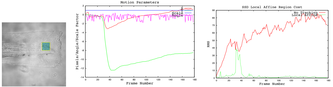
Fig. 2. Analysis of frame-to-frame local affine texture tracking errors. The region marked on the left image (on Frame 1), was tracked over the entire sequence of 180 frames. The middle plot shows the transformation parameters: cumulative shift (x - red, y - green), differential scale (blue) and angle (magenta). The right plot shows the mean squared error between the first frame and subsequent frames with and without compensating for the block motion. The registration error (green line) remains small and fairly constant other than for a small period between frames 35 and 40 where a violent motion is non-linear within the tracked region (of size 32). The error without motion compensation (red line) continues to grow.
