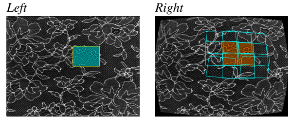
Fig. 1. Example illustrating local affine region matching. The target image (labelled Right) has been synthetically warped with a barrel deformation. The local affine transformation for a single region and its overlapping neighbours, size 128 \times 128 pixels is shown. The pixels in blue on the Left image are taken from corresponding pixels in the target frame (Right), and those in orange on the Right image from the source.
