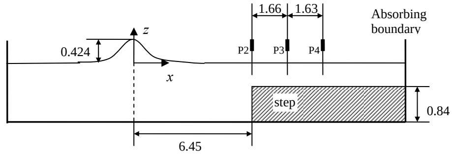
Fig. 7 Sketch of the configuration for the case with a submerged step
