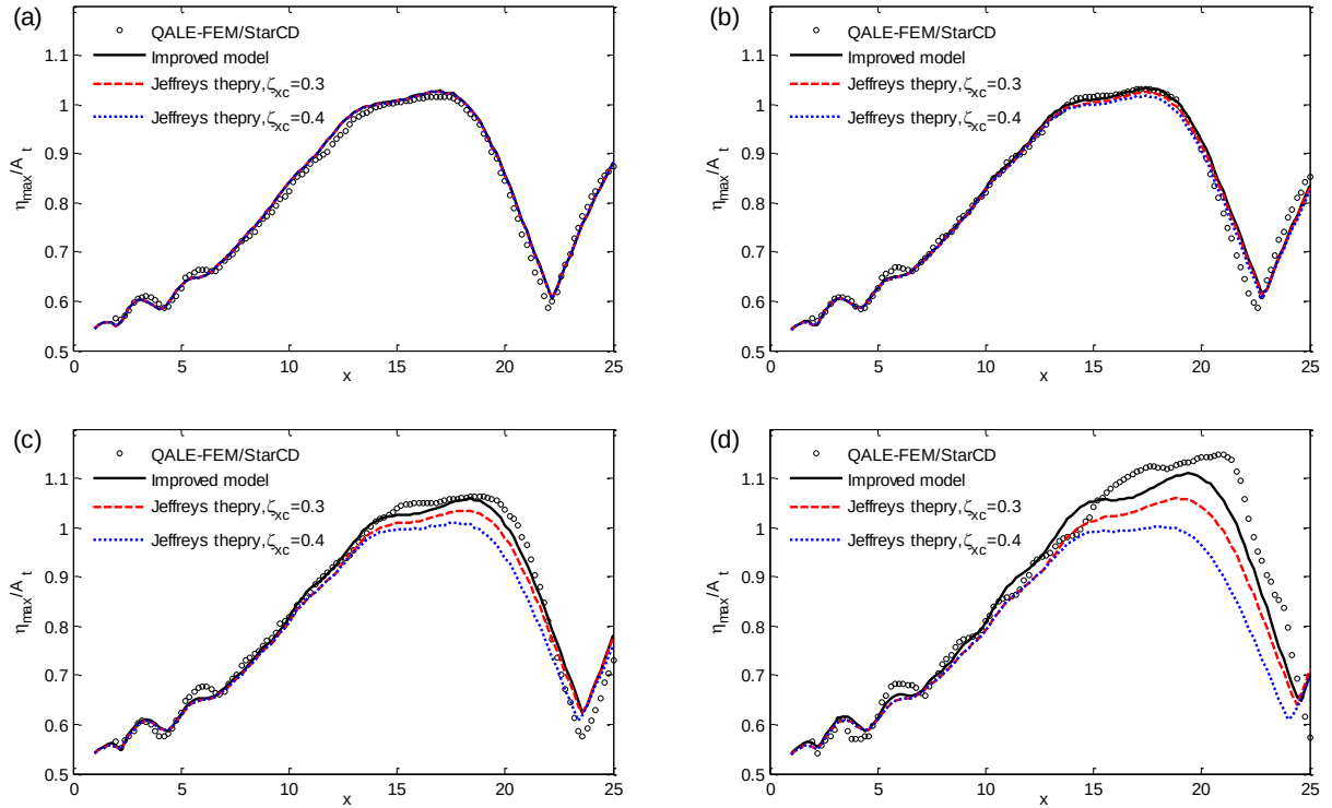
Fig. 13 Comparison of maximum elevation recorded at different positions for (a) U_w = 0.958 ; (b) U_w = 1.916 ; (c) U_w = 2.874 and (d) U_w = 3.832 ( \omega_{min} = 0.5 , \omega_{max} = 1.4 , N=32 , a_n=0.008 , x_f=12.5 , \tau_f=46.97 )
