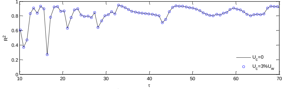
Fig.4 Square of correlation coefficient ( R^2 ) at different time steps ( \omega_{\min} = 0.5 , \omega_{\max} = 1.4 , N=32 , a_n = 0.008 , x_f=10 , \tau_f=31.32 , U_w=2.874 , l_l=(c_{g\max} - c_{g\min})\tau_f/2 )
