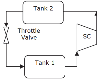
Figure 1: Two Tanks schematics
