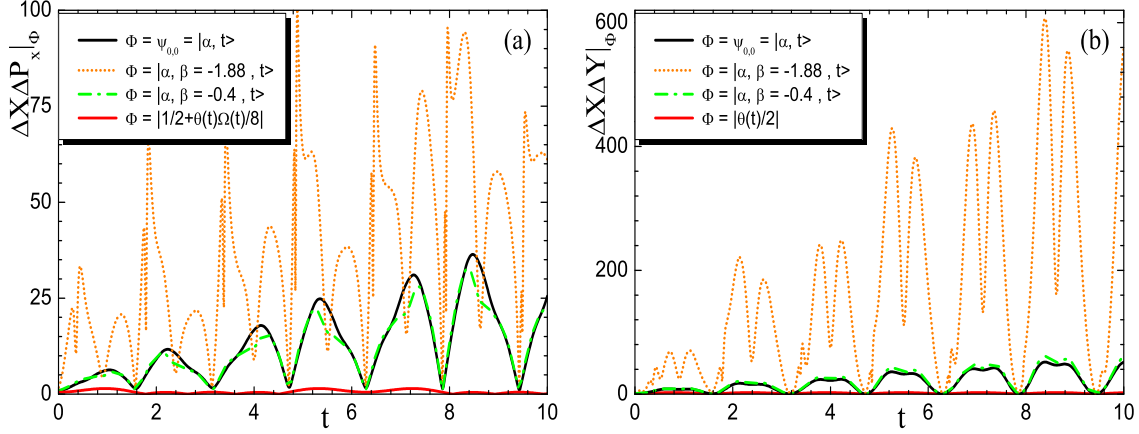
Figure 6: Uncertainties with respect to Glauber coherent states versus squeezed Glauber coherent states for the noncommutative variables X, Y, P_x for background fields \theta(t) = \alpha \sin(\gamma t) and \Omega(t) = \beta \sin(\gamma t/2) . In both panels the constants are \alpha = 5 , \beta = 2 , \gamma = 2 , m = \hbar = \tau = \omega = 1 , \kappa = 1/4 and \mu = \sqrt{5/3} .
