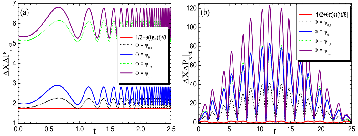
Figure 4: Uncertainties \Delta X \Delta P_x|_{\psi_{n,m-n}} versus the generalized lower bound (a) for background fields \theta(t) = \alpha e^{-\gamma t} and \Omega(t) = \beta e^{\gamma t} and (b) for background fields \theta(t) = \alpha \sin(\gamma t) and \Omega(t) = \beta \sin(\gamma t/2) . In both panels the constants are \alpha = 5 , \beta = 2 , \gamma = 2 , m = \hbar = \tau = \omega = 1 , \kappa = 1/4 and \mu = \sqrt{5/3} .
