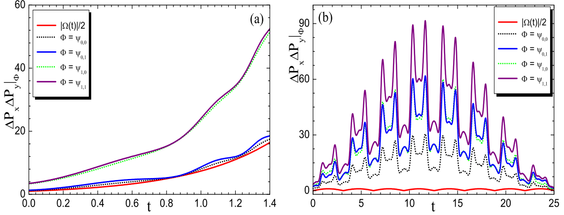
Figure 3: Uncertainties \Delta P_x \Delta P_y|_{\psi_{n,m-n}} versus the generalized lower bound (a) for background fields \theta(t) = \alpha e^{-\gamma t} and \Omega(t) = \beta e^{\gamma t} and (b) for background fields \theta(t) = \alpha \sin(\gamma t) and \Omega(t) = \beta \sin(\gamma t/2) . In both panels the constants are \alpha = 5 , \beta = 2 , \gamma = 2 , m = \hbar = \tau = \omega = 1 , \kappa = 1/4 and \mu = \sqrt{5/3} .
