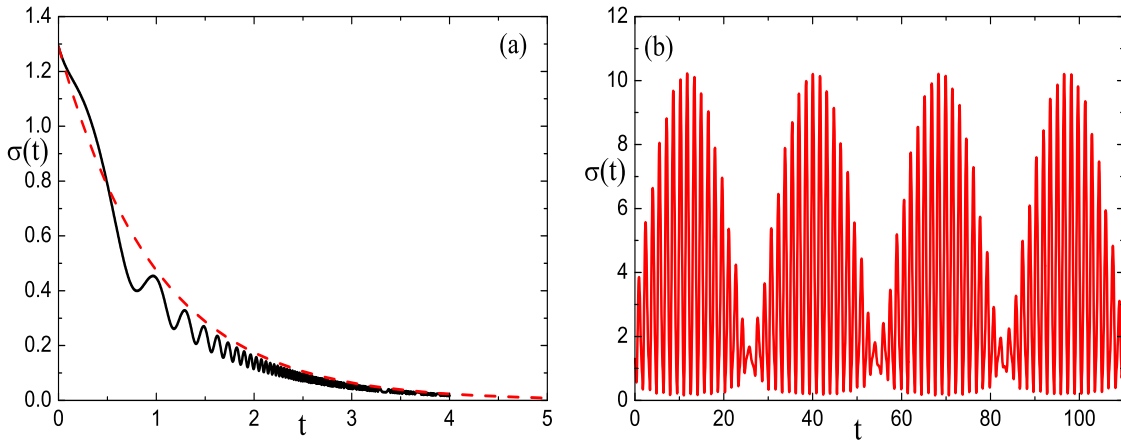
Figure 1: (a) Exactly integrable solution (3.13) (red, dashed) versus a non-Chiellini integrable solution for pre-selected exponential backgrounds \theta(t) = \alpha e^{-\gamma t} and \Omega(t) = \beta e^{\gamma t} (black, solid). (b) Non-Chiellini integrable solution for pre-selected sinusoidal background \theta(t) = \alpha \sin(\gamma t) and \Omega(t) = \beta \sin(\gamma t/2) . In both panels the constants are \alpha = 5 , \beta = 2 , \gamma = 2 , m = \hbar = \tau = \omega = 1 , \kappa = 1/4 and \mu = \sqrt{5/3} .
