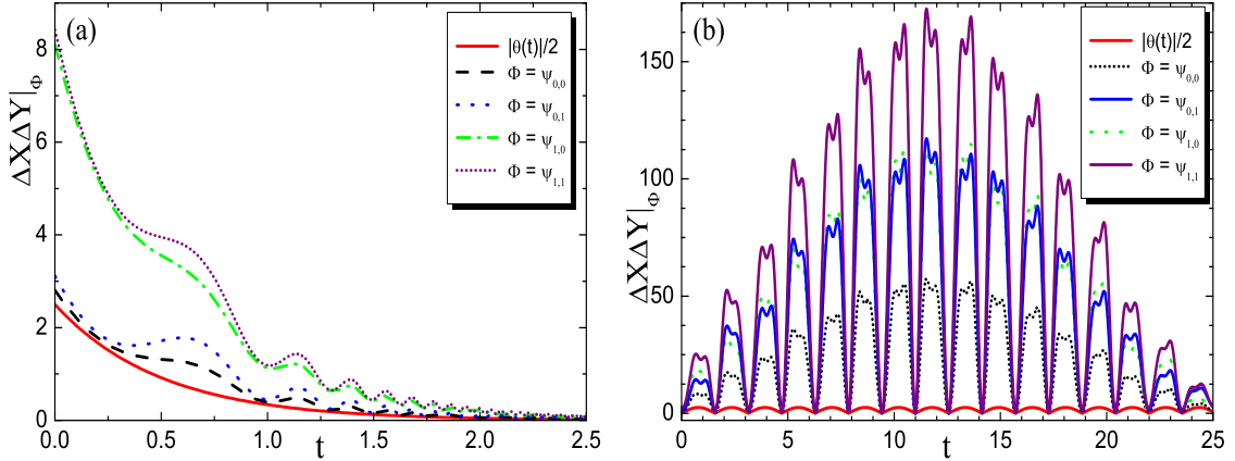
Figure 2: Uncertainties \Delta X \Delta Y|_{\psi_{n,m-n}} versus the generalized lower bound (a) for background fields \theta(t) = \alpha e^{-\gamma t} and \Omega(t) = \beta e^{\gamma t} and (b) for background fields \theta(t) = \alpha \sin(\gamma t) and \Omega(t) = \beta \sin(\gamma t/2) . In both panels the constants are \alpha = 5 , \beta = 2 , \gamma = 2 , m = \hbar = \tau = \omega = 1 , \kappa = 1/4 and \mu = \sqrt{5/3} .
