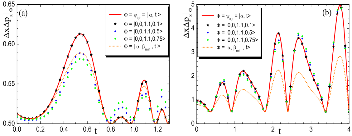
Figure 5: Uncertainties with respect to Glauber coherent states versus squeezed Glauber coherent states and Gaussian Klauder coherent states for the auxiliary variables x, p_x , \Delta x \Delta p_x|_{|\alpha,t\rangle} versus \Delta x \Delta p_x|_{|\alpha,\beta,t\rangle} versus \Delta x \Delta p_x|_{|GK\rangle} (a) for background fields \theta(t) = \alpha e^{-\gamma t} and \Omega(t) = \beta e^{\gamma t} and (b) for background fields \theta(t) = \alpha \sin(\gamma t) and \Omega(t) = \beta \sin(\gamma t/2) . In both panels the constants are \alpha = 5 , \beta = 2 , \gamma = 2 , m = \hbar = \tau = \omega = 1 , \kappa = 1/4 and \mu = \sqrt{5/3} .
