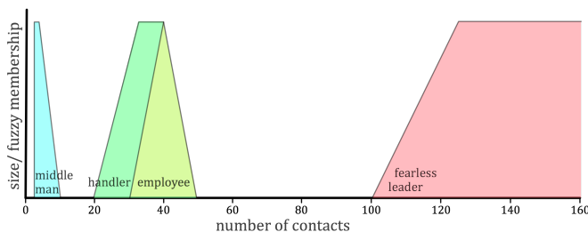
Figure 4: Node size rules for categorized Flitter users
