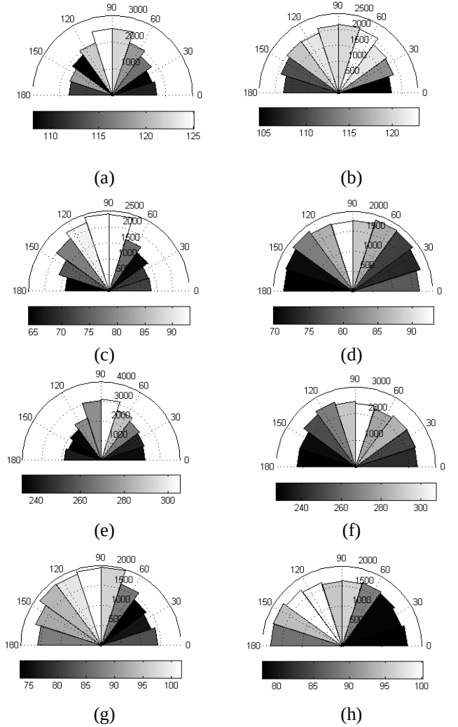
Figure 4. Rose diagrams for specimens at load stage 4 (shading indicates average contact area in \mu\text{m}^2 ); (a) CN Int-3a; (b) BV Int-3a; (c) CN Rec-3aS; (d) BV Rec-3aS; (e) CN Int-4bS; (f) BV Int-4bS; (g) CN Rec-4aS; (h) BV Rec-4aS
