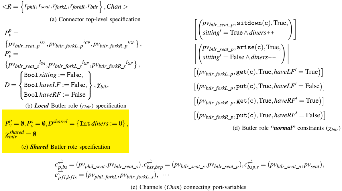
Figure 6: Centralized dining philosophers connector
