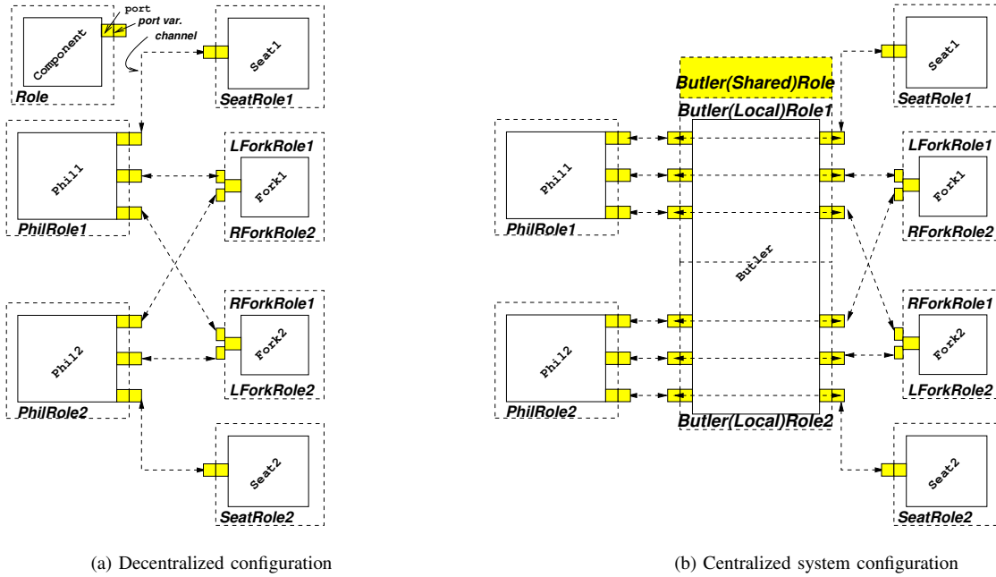
Figure 9: System configurations
