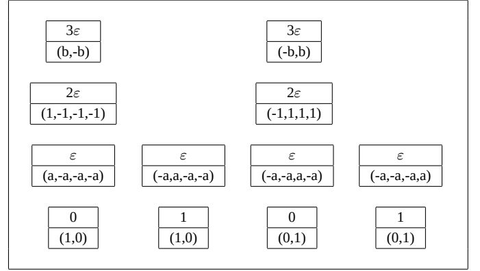
Rows indicate layers (from bottom up). Boxes indicate neurons; rows inside boxes indicate input weights and context weights. Note that only context weights referring to neurons from previous layer are displayed; all other context weights are 0, as the activation of these neurons is close to 0 as well.
