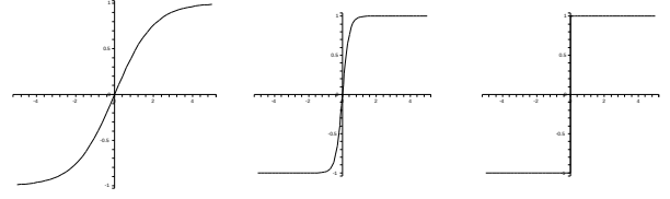
Figure 7: With increasing z , \sigma_{l,h,m,z} gets arbitrarily close to s_{l,h,m} everywhere but at m . The difference between \sigma_{l,h,m,z} and s_{l,h,m} is symmetric to m and decreases with increasing distance from m . Shown here are \sigma_{-1,2,0,1} , \sigma_{-1,2,0,5} , s_{-1,2,0} .
