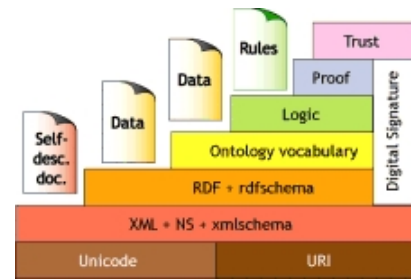
Figure 1: The Semantic Web Layer Cake
