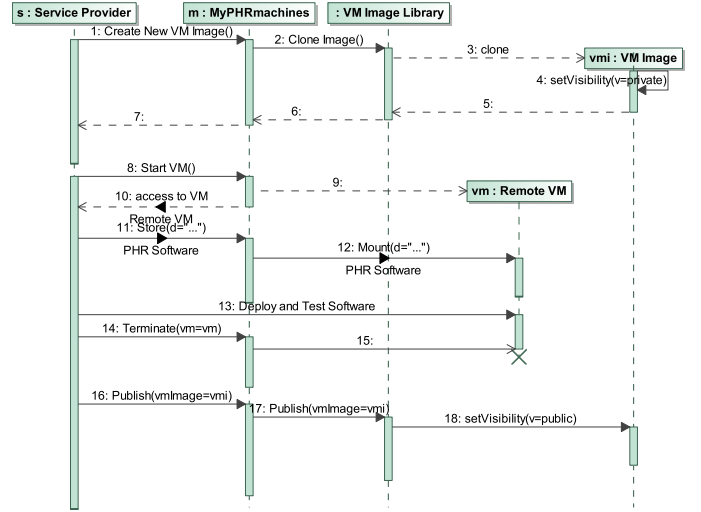
Fig. 5. Deploying a new software service in MyPHRMachines.
