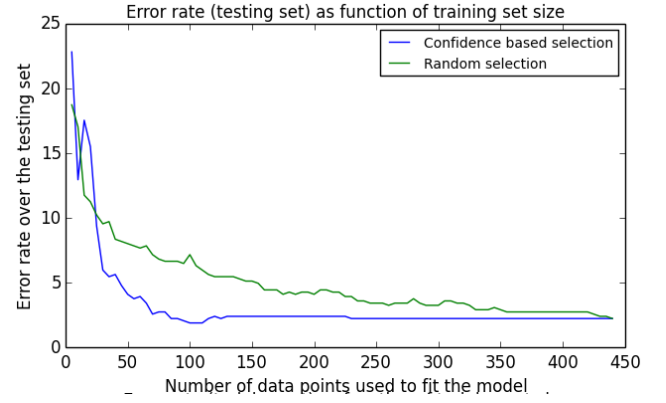
Figure 4: Test set performance of SVM. The bottom blue curve corresponds to uncertainty sampling, the top green curve measures random sampling.
