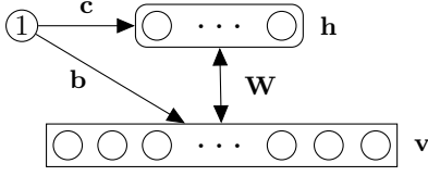
Figure 2: A simple Restricted Boltzmann Machine with four visible, two hidden, and no bias units.
