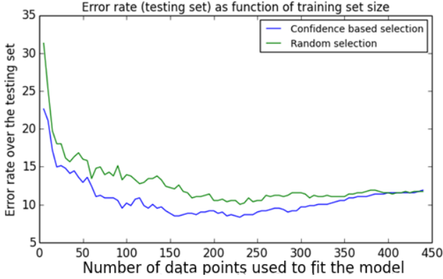
Figure 6: Performance of the audio features for random and uncertainty sampling. The performance is relatively low in both cases.
