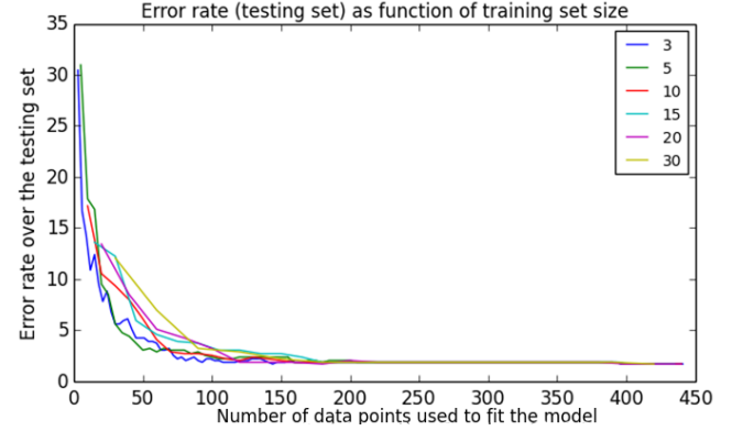
Figure 8: Comparison of different increment sizes over growing training sets. Smaller increments show better performance with few training data.
