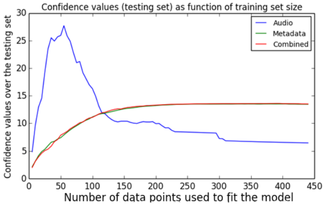
Figure 7: Comparison of feature types’ effects on the confidence of test set classifications. Audio features perform badly with large training sets.
