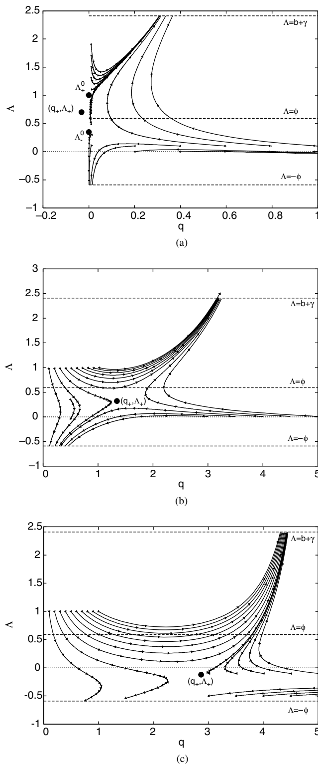
Figure 5 Phase Diagrams for Optimal Premium Strategy in a Finite Market and Terminal Wealth Objective with q_m = 5
