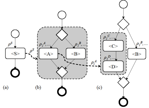
Figure 2: Recursive application of secure service orchestration patterns.
