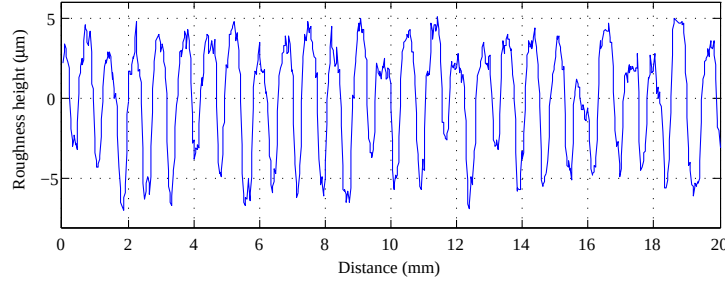
Figure 5: Measured surface roughness of PCB2
