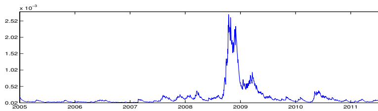
(c) Conditional variance for S&amp;P 500
