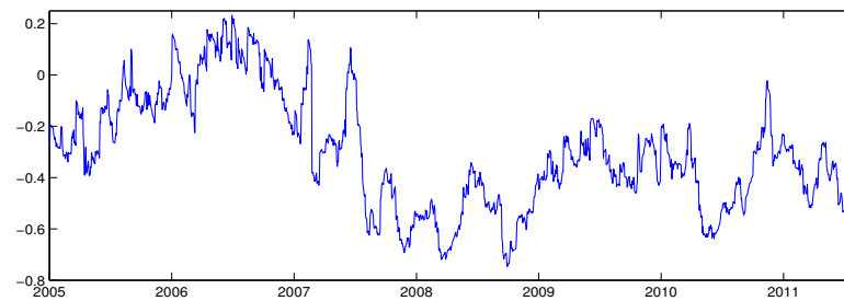
(b) Conditional correlation S&amp;P 500 and SHY
