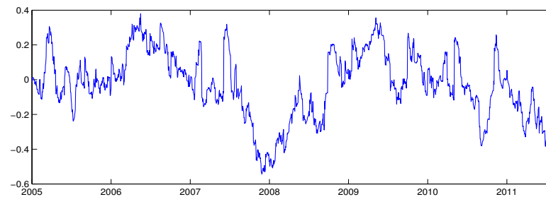
(c) Conditional correlation S&amp;P 500 and LQD
