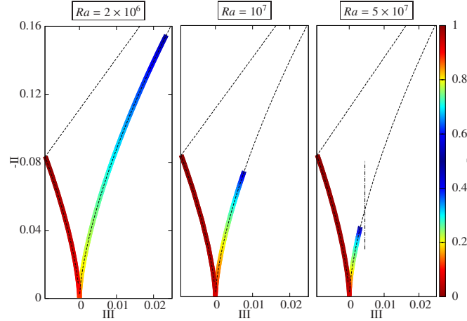
FIG. 8. Invariants of the deviatoric part of the Reynolds stress tensor plotted in a so-called Lumley map for cases C1, C3 and C5. Red corresponds to the region close to the boundaries whereas blue corresponds to the middle of the layer. From left to right, the Rayleigh number is increasing. The vertical dash-dotted line in the right panel correspond to the approximate critical value of the invariant III below which the flow cannot sustain a 2D mode.
