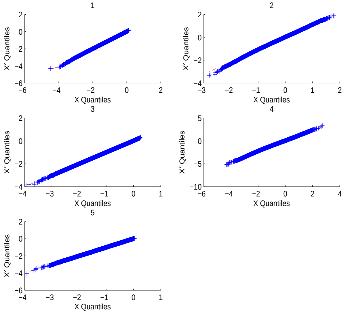
Figure 5 Convolution error: recovering the VG distribution. 5 Assets
