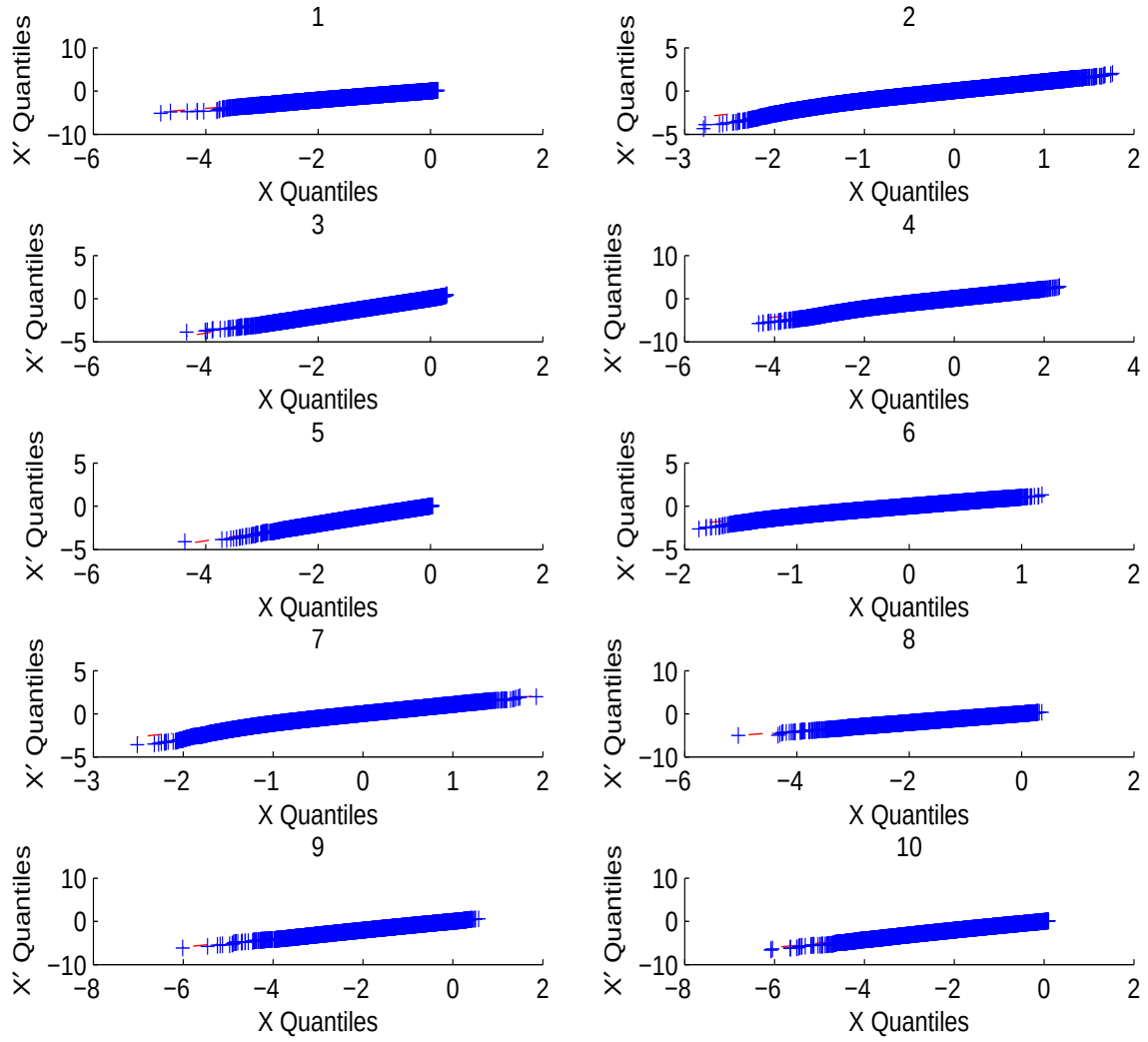
Figure 6 Convolution error: recovering the VG distribution. 10 Assets
