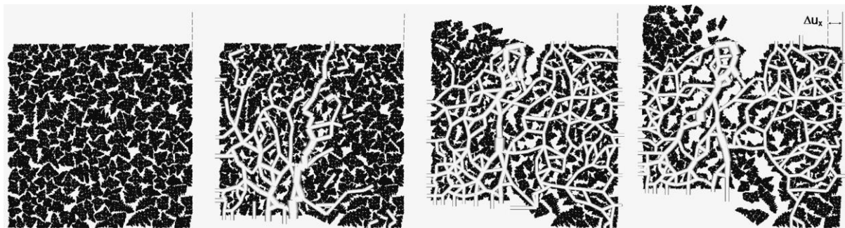
Figure 9. Two-dimensional DEM simulation of shear-induced dilation in an equiaxed-dendritic microstructure deformed in direct shear. The left hand side wall is stationary and a constant stress condition has been applied to the right-hand side wall such that it adjusts its horizontal displacement to maintain a constant stress. Dashed black lines are the initial right-hand wall position and solid black lines are the current position. The white lines are force chains with line thickness proportional to force magnitude. Force is transmitted across crystal–crystal contacts and shear-induced dilation \Delta u_z emerges naturally from the simulation. Full details are given in Ref. 33.
