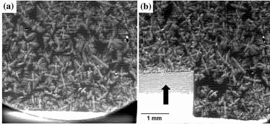
Figure 7. Radiographs of Al-15Cu with equiaxed-dendritic morphology at ~30% solid: (a) prior to deformation and (b) after 1606 \mu\text{m} (3.8 mean grains) of push-plate displacement.
