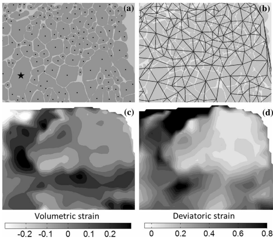
Figure 6. (a) Separated grains and their centroids from part of Fig 5a. The centroid marked with a star is the grain highlighted in Figure 5. (b) Delaunay triangulation of the centroids. (c) Volumetric strain field where positive values indicate dilation. (d) Deviatoric strain field. The strain fields have been smoothed and are for the deformation increment from Figure 5(a) and (b).
