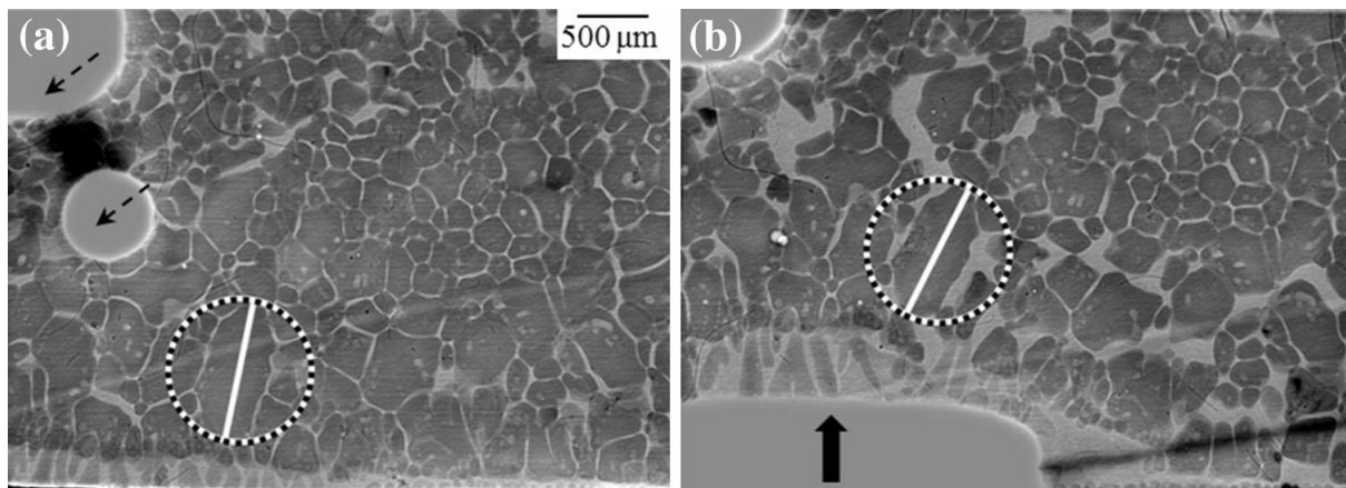
Figure 5. Deformation of globular–polygonal Fe-2C-1Mn-0.5Si at ~88% solid: (a) prior to deformation and (b) after 1072 \mu\text{m} (3.1 mean grains) of push-plate displacement. Note the significantly enlarged liquid-filled interstices in (b) due to shear-induced dilation. The primary axis and circle of rotation are shown for a large grain with high aspect ratio. Austenite is dark gray, liquid is light gray, and the rounded features marked with arrows are pores.
