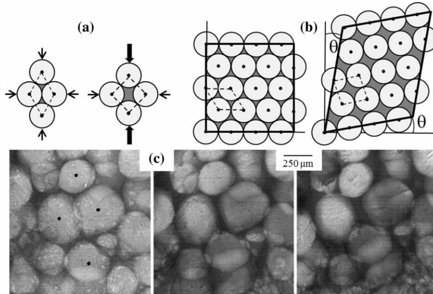
Figure 2. (a, b) Shear-induced dilation of ordered close-packed circles: (a) four circles in biaxial compression and (b) 20 circles in pure shear. Grains are light gray, grain centroids are marked with dots, interstitial liquid is shaded dark grey and arrows indicate the direction and magnitude of force. (c) Four globules in Al-15Cu at ~70% solid (centroids marked with dots) loaded similar to (a).
