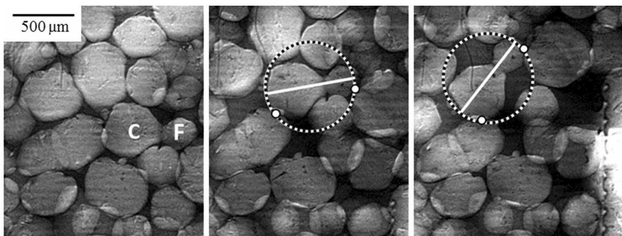
Figure 4. Deformation of globular Al-15Cu at ~70% solid, highlighting the role of the rotation of an agglomerate of grains C and F with bowling pin shape. White dots mark the contacts important in causing rotation, white lines are the primary axis of the agglomerate formed by grains C and F, and the dashed line is the circle with diameter equal to the primary axis of the agglomerate. The push plate can be seen to the far right of each image.
