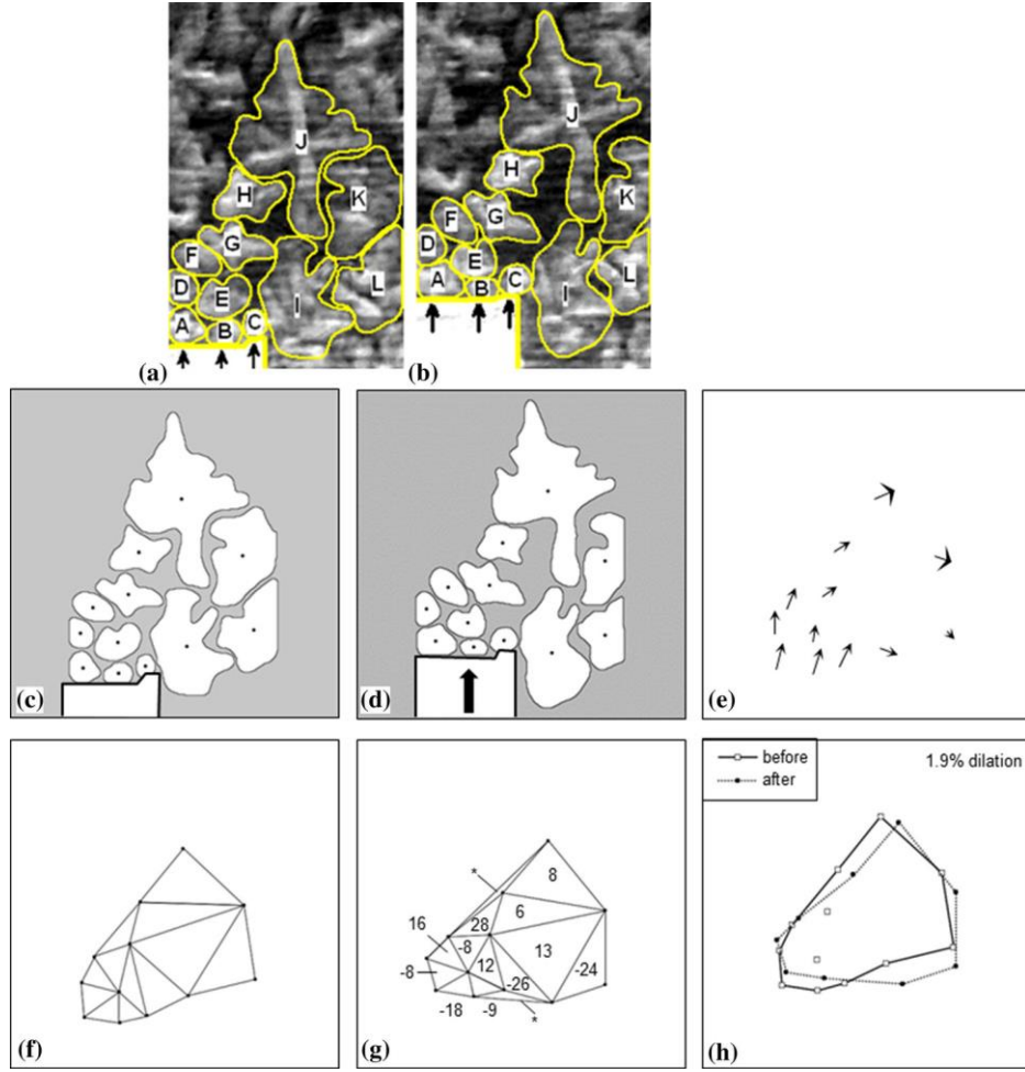
Figure 8. Local region of shear-induced dilation in equiaxed-dendritic Al-15Cu at ~30% solid. (a, b): Radiographs of 12 crystals with envelopes estimated in yellow. (c and d): Projected-area envelope outlines and centroids. (e) Centroid displacements from (c) to (d). (f and g): Triangulation of the globule centroids. The values in (g) are the % volumetric strain of the triangles. (h) Overall area change of the centroid polygons = 1.9% dilation.
