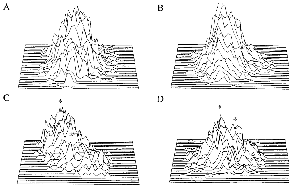
Figure 7. Three-dimensional representations of event-type MURFs recorded in ( A , C ) normal and ( B , D ) strobe-reared frogs. The x - and y -axes correspond to 64.5° of the nasotemporal and 34.5° of the superoinferior visual field, equivalent to the area covered by the television monitor on which the MURFs were plotted. The z -axis represents the cumulative number of spikes recorded in each 1.5 \times 1.5 pixel on the screen from three traverses in each orthogonal direction from which the MURF areas were measured. Asterisks ( C , D ) denote double activation peaks.
