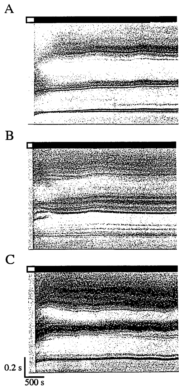
Figure 3. Entrained patterns of RGC firing induced by exposure to a continuous 1 Hz of stroboscopic illumination in ( A ) sustained, ( B ) event, and ( C ) dimmer unit classes. In these raster plots each dot represents an action potential recorded during the first 3 hr of an uninterrupted recording session in three different experiments ( A , B , and C ; one of the unit pairs str-03, str-02, and str-07). The x-axes represent the time (in seconds) for this part of each recording session, and the y-axes correspond to the 1 sec interval between strobe flashes (occurring at the abscissa in each plot). For the period indicated by the short open bar at the top of each panel, the frog was maintained in darkness while spontaneous discharges were monitored; the long black bar indicates the period of exposure to stroboscopic illumination. Within a few minutes of strobe onset, an entrained triphasic response pattern emerges and is maintained throughout the recording period. Calibration (bottom left) refers to all panels.
