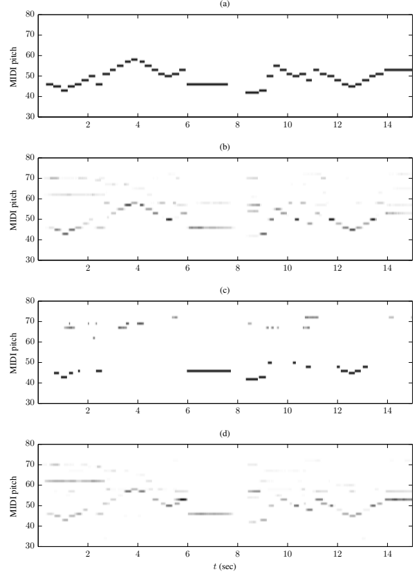
Fig. 1. Piano-roll representations for the bassoon track of recording “Herr Gott” from the Bach10 dataset. (a) Ground-truth. (b) Output of the AMT system. (c) Output of the instrument recognition system. (d) Output of the integrated system.
