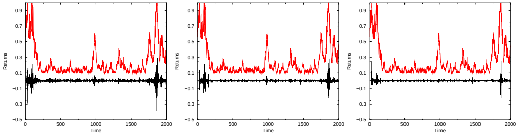
Fig. 2. Returns time series with a time dependent \lambda and w=0.2 (left), w=0.5 (center) and w=0.8 (right). The evolution of p is described by the red line.
