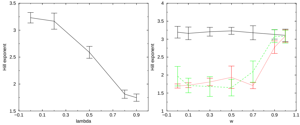
Fig. 3. Hill exponents of the returns distribution as as a function of constant \lambda for w = 0.5 (left side). Hill exponents of the returns distribution as a function of w for \lambda = 0 , \lambda = 1 and \lambda time dependent, respectively black, red and green lines (right side).
