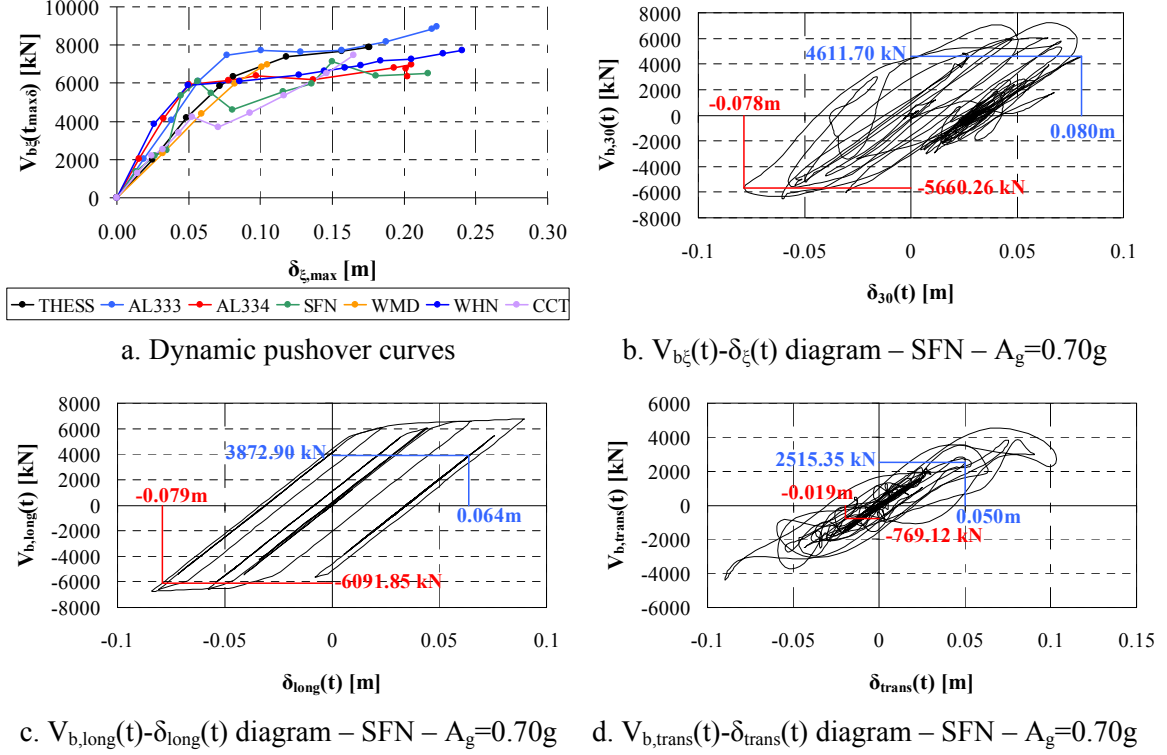
Figure 12. Dynamic response of the bridge – Bidirectional excitation, a = 30^\circ
