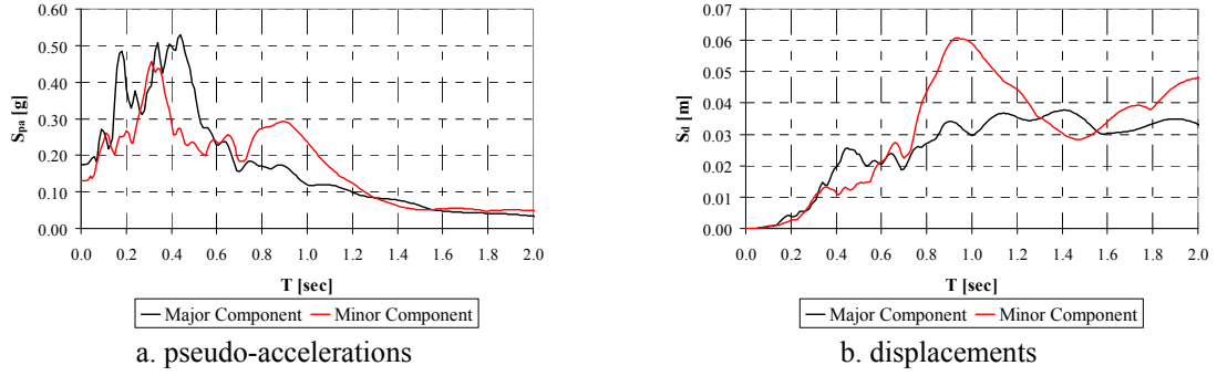
Figure 7. Elastic response spectra for principal components of Thessaloniki record
