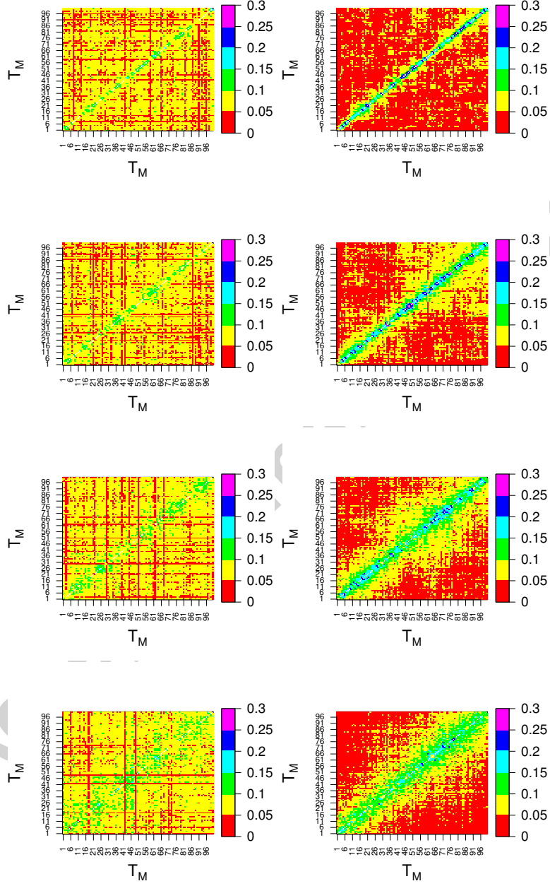
Figure 3: Weighted Jaccard index matrices for the lender-aggressor simulated networks (left panels) and the corresponding validated networks (right panels). The networks are obtained from simulation with values for the memory parameter, from top to bottom, Q = 1 , Q = 2 , Q = 4 and Q = 8 . The randomization parameter w is equal to 1 in all the simulations showed.
