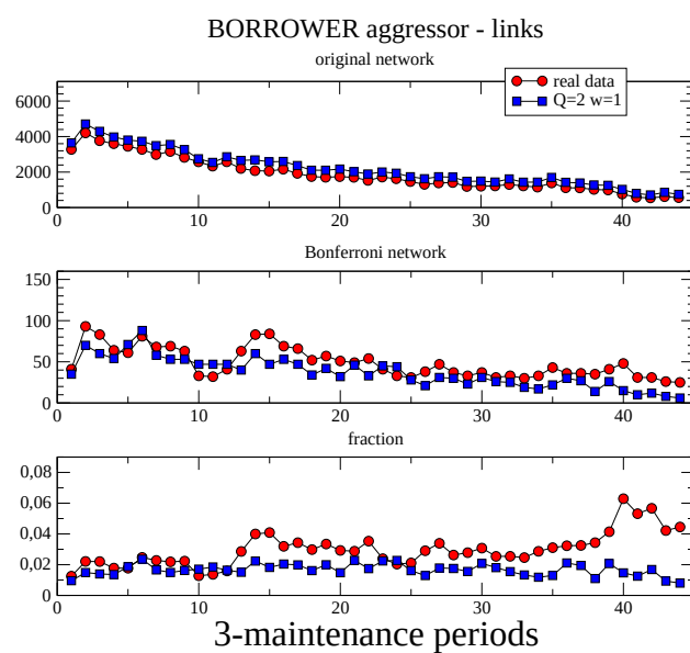
Figure 7: Number of links in the original (top) and Bonferroni (central) network associated with borrower-aggressor transactions simulated according to the presented model, for w = 1 ad Q = 2 . The red circles refer to the empirical data. The bottom panel shows the ratio between number of links in the Bonferroni and original network.
