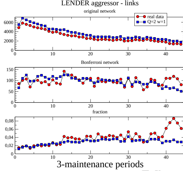
Figure 6: Number of links in the original (top) and Bonferroni (central) network associated with lender-aggressor transactions simulated according to the presented model, for w = 1 and Q = 2 . The red circles refer to the empirical data. The bottom panel shows the ratio between number of links in the Bonferroni and original network.
