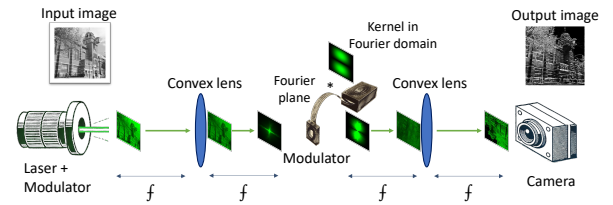
Fig. 1. Schematic illustration of a 4f optical system executing a convolution operation. The system consists of an input plane (laser source), a convex lens, and a Fourier plane (containing a modulator or phase mask), followed by another convex lens and a camera, each positioned one focal length away from the lenses. As the light passes through the first lens, it undergoes a 2D Fourier transform at the Fourier plane, where it is multiplied by the kernel in the frequency domain. The light then travels through the second lens, which transforms it back to the spatial domain, and the camera captures the output.
