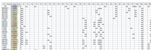
FIGURE 1. Fragment of table-based rule visualization. Each row corresponds to a rule. The first four columns show rule and tree identifiers, predicted potency, and number of conditions; the remaining columns are binary fingerprint features, left-aligned for absent (0) and right-aligned for present (1).
