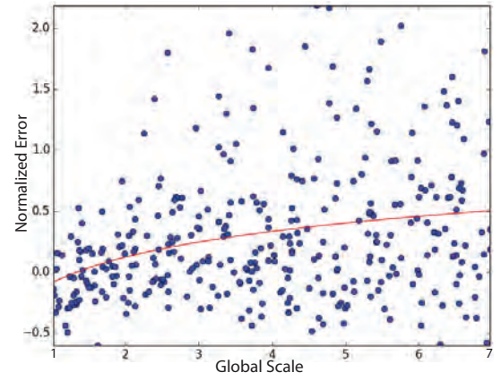
Fig. 9: Error distribution computed following Steven's power law vs. the global scale test parameter.
