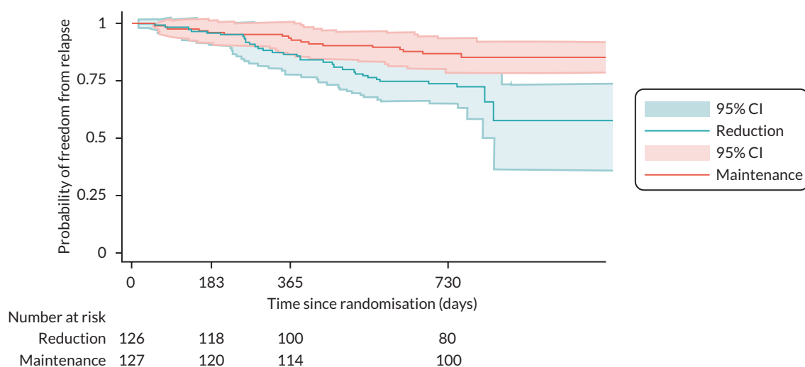
FIGURE 4 Kaplan-Meier curve.
