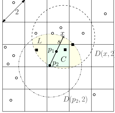
■ Figure 3 The cell C is represented by the light-blue colored cell with p_1, p_2 \in C . The thick black line denotes the line segment s = \overline{p_2 x} of length 2, passing through p_1 . The dotted disk represents D(x, 2) , while the dash-dotted disk represents D(p_2, 2) . The yellow-shaded region corresponds to the lens L = D(x, 2) \cap D(p_2, 2) , formed along the axis s .
