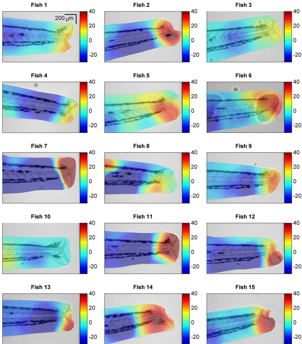
Figure 6. Chemoattractant field inference in the zebrafish. For each zebrafish, 1–15, the estimate of the chemoattractant field (colour) is overlaid with transparency on the fish image (grayscale). Each colormap is scaled to the range -20 to 40 to provide an effective visual comparison over all fish. The chemoattractant field estimate is dimensionless hence the scale of the colormap is in arbitrary units. doi:10.1371/journal.pone.0035182.g006
