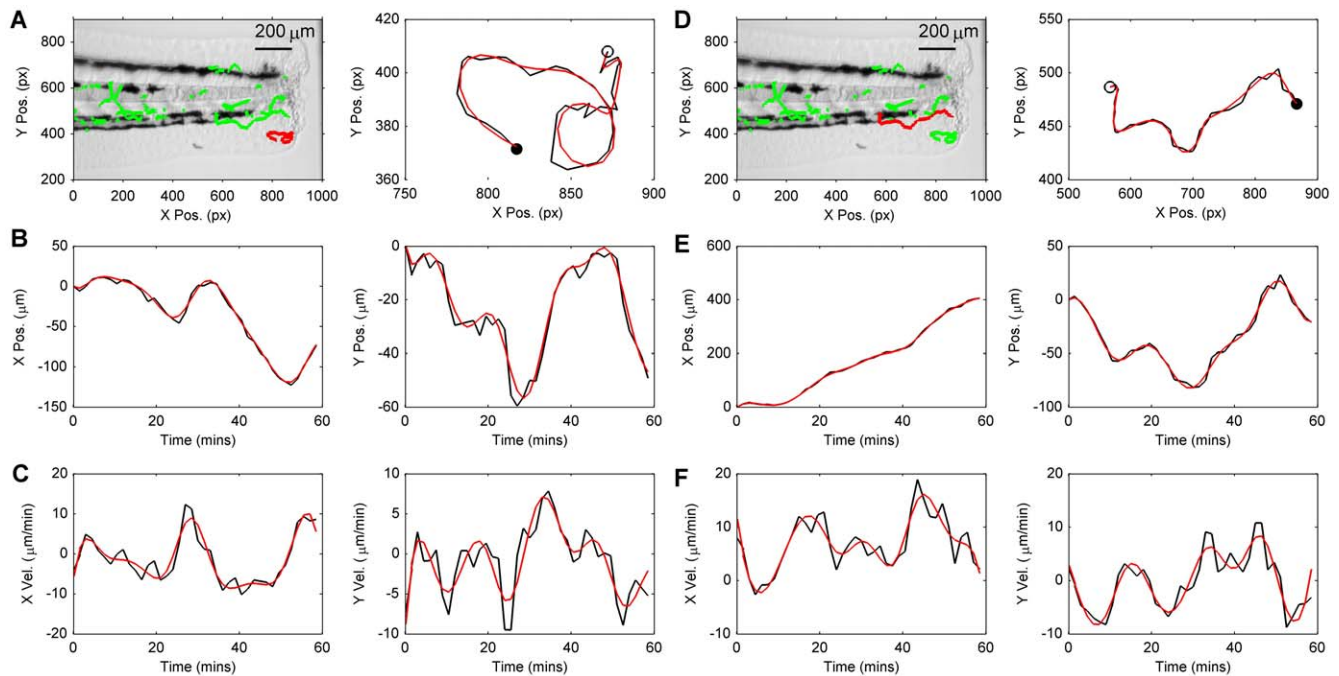
Figure 3. Typical examples of neutrophil tracks and neutrophil velocity estimates. A and D: The image on the left shows a highlighted red track that is zoomed in the plot on the right, in which the centroid positions extracted from the tracking algorithm (black) and smoothed track estimate (red) are compared (the open circle indicates the track start point and the filled circle indicates the track end point). B and E: X-Y cell centroid position estimates corresponding to tracks highlighted in A and D are shown as signals with respect to time produced by the tracking algorithm (black) and estimates from the smoothing algorithm (red). C and F: X-Y velocity estimates (raw estimates in black and smoothed estimates in red), corresponding to position signals in B and E. Raw estimates of velocity were obtained by numerical differencing (central difference method) applied to the tracker position estimates.
