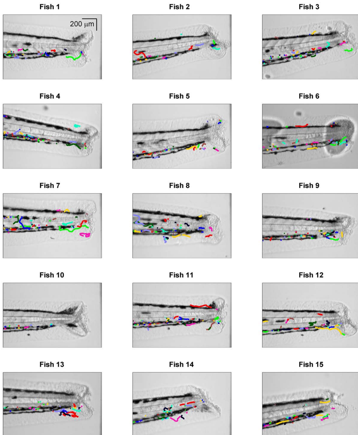
Figure 2. Neutrophil centroid position tracks. The neutrophil tracks (colour lines) were obtained from a segmentation and tracking algorithm and are shown here in relation to the zebrafish image (greyscale), where the zebrafish image of dimension 1000 \times 1000 pixels has been zoomed on the vertical axis to the 100–900 pixel range. doi:10.1371/journal.pone.0035182.g002
