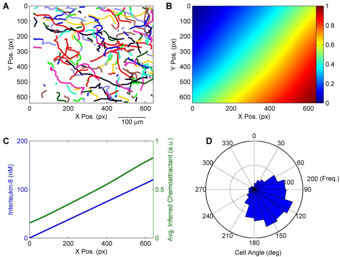
Figure 5. Chemoattractant field inference in vitro . A: Cell tracks of human neutrophils in vitro chemotaxing due to presence of the chemokine interleukin-8, which increases in concentration from left to right. B: Inferred chemoattractant field, normalised to the range (0,1). The chemoattractant field estimate is dimensionless hence the scale of the colormap is in arbitrary units (a.u.). C: Comparison of inferred chemoattractant field averaged over the Y-direction, to the level of chemokine interleukin-8 reported in [30]. D: Circular histogram of neutrophil angles, demonstrating a directional bias of the tracks shown in panel A towards the lower right corner. doi:10.1371/journal.pone.0035182.g005
