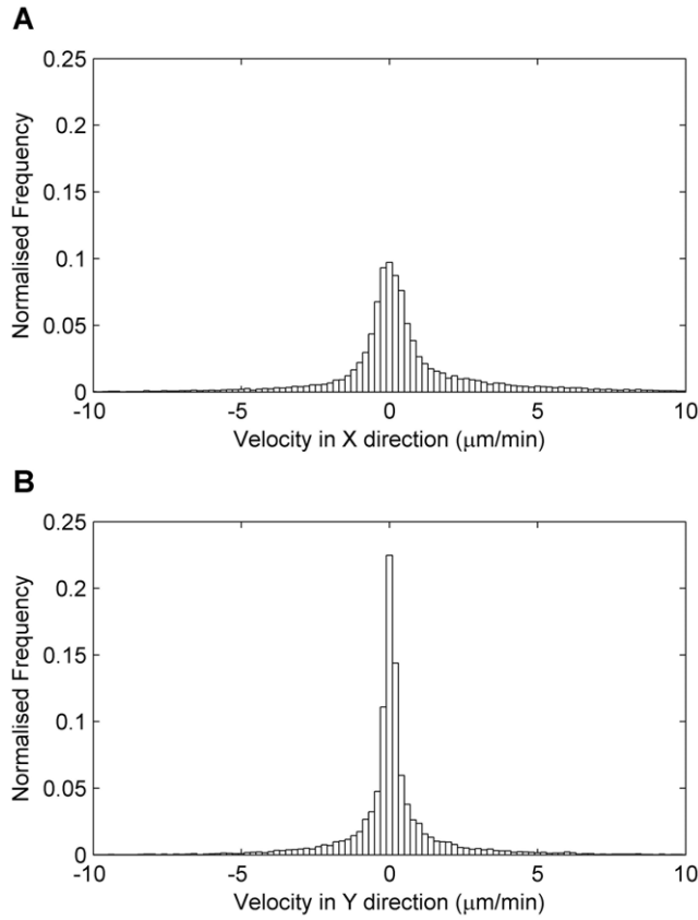
Figure 4. Neutrophil velocities. A: Histogram of neutrophil velocities in the X-direction at each sample time (histograms are zoomed to the -10 to 10 \mu\text{m}/\text{min} range for an effective visualisation and data are aggregated over all fish). B: Histogram of neutrophil velocities in the Y-direction. doi:10.1371/journal.pone.0035182.g004
