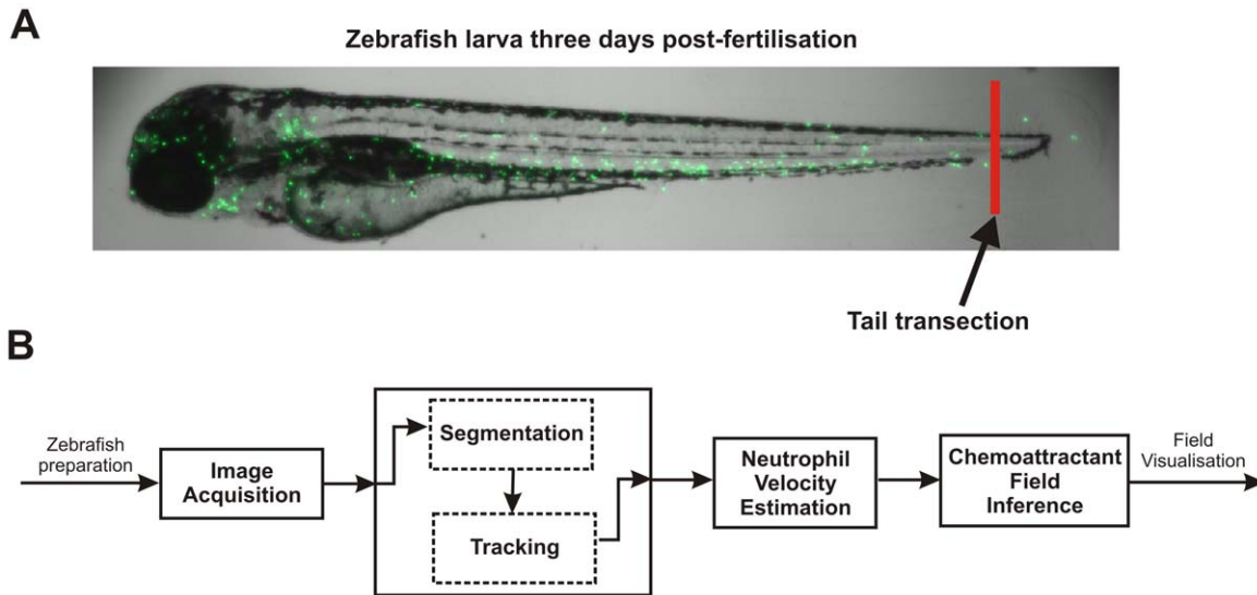
Figure 1. Zebrafish experimental setup and neutrophil analysis procedure. A: Zebrafish larva from the transgenic line, Tg(mpx:GFP)i114. Neutrophils are visualised by excitation of green fluorescent protein, as previously described (Renshaw et al., 2006). The zebrafish were prepared by transection of the tailfin at the site indicated to elicit an inflammatory response, which caused recruitment of the neutrophils to the site of injury. B: The chemoattractant field inference framework. Firstly, images of neutrophil recruitment to the zebrafish wound site were acquired by video microscopy. The neutrophil centroid positions were then obtained from a segmentation and tracking algorithm. Velocities of the neutrophils were estimated from the neutrophil centroid tracks using a Kalman smoother and lastly, the velocity estimates were used in the inference of the chemoattractant field. doi:10.1371/journal.pone.0035182.g001
