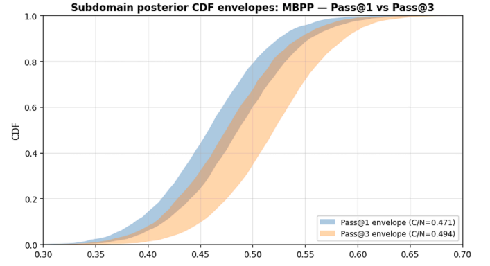
Fig. 9. Subdomain-level posterior CDF envelopes of non-failure probability for MBPP under alternative success definitions. Results are shown for Claude Sonnet 4.5 on MBPP ( N = 257 ), using identical tasks, prompts, and tests. Pass@1 yields \frac{C}{N} = 0.471 , while Pass@3 yields \frac{C}{N} = 0.494 . Envelopes reflect imprecise hierarchical inference with identical hyper-hyperparameter intervals; only the success definition differs. A question-oriented interpretation of figure: how does the inferred subdomain-level non-failure probability change when alternative success (failure) definitions, such as Pass@1 versus Pass@3, are used on the same evaluation data?
