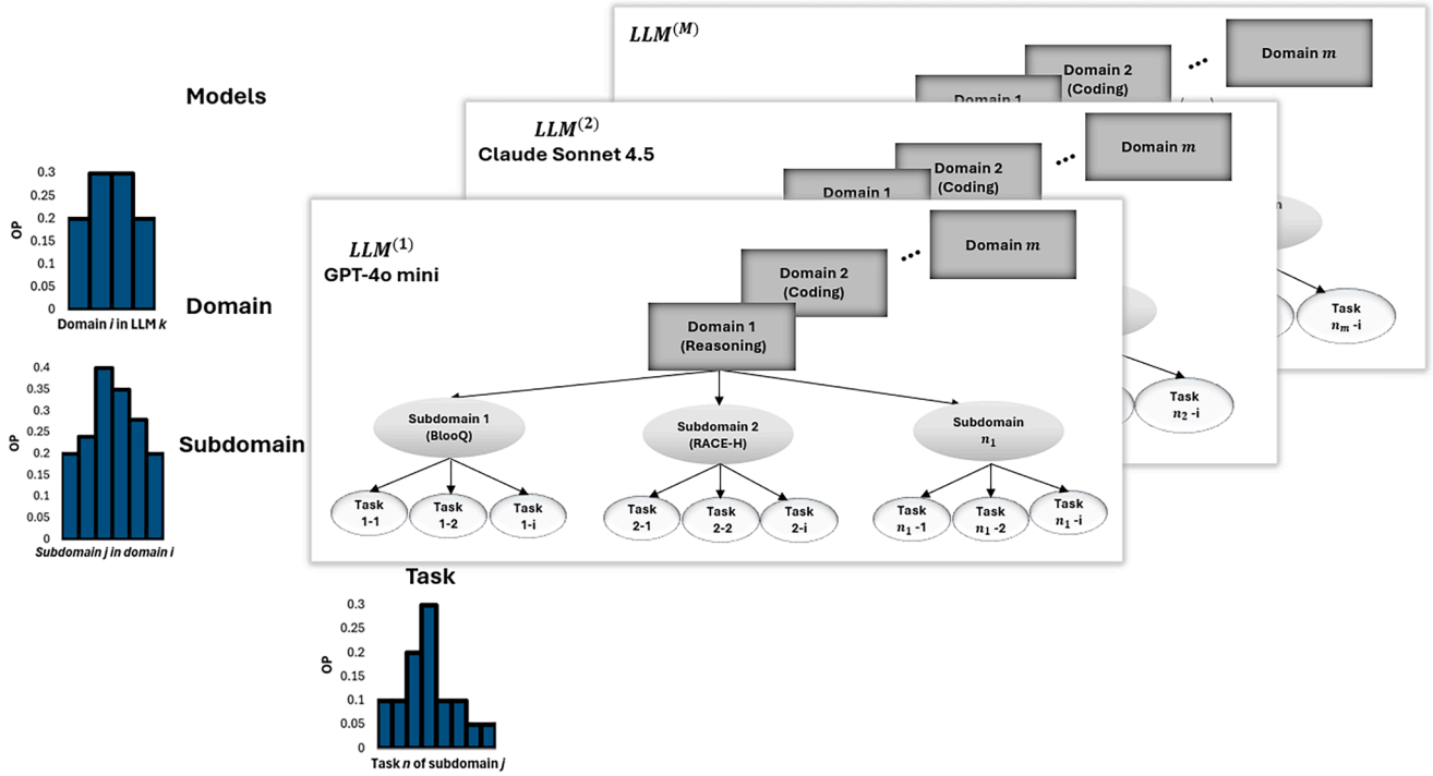
Fig. 1. Schematic representation of the hierarchical LLM, domain, and subdomain structure for reliability estimation for M LLM models. Rectangles indicate independent components, while ovals indicate dependent components within the hierarchy.
