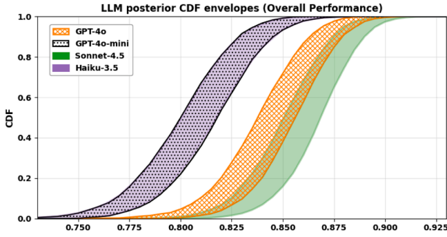
Fig. 5. Posterior CDF envelope of non-failure probability of overall LLM level ( p_L = \sum_i W_i p_i ) with domain weights W = (0.149, 0.851) across four models. A question-oriented interpretation of figure: Engineering question: After observing the evaluation data, how do the four LLMs differ in terms of their LLM-level non-failure probability?
