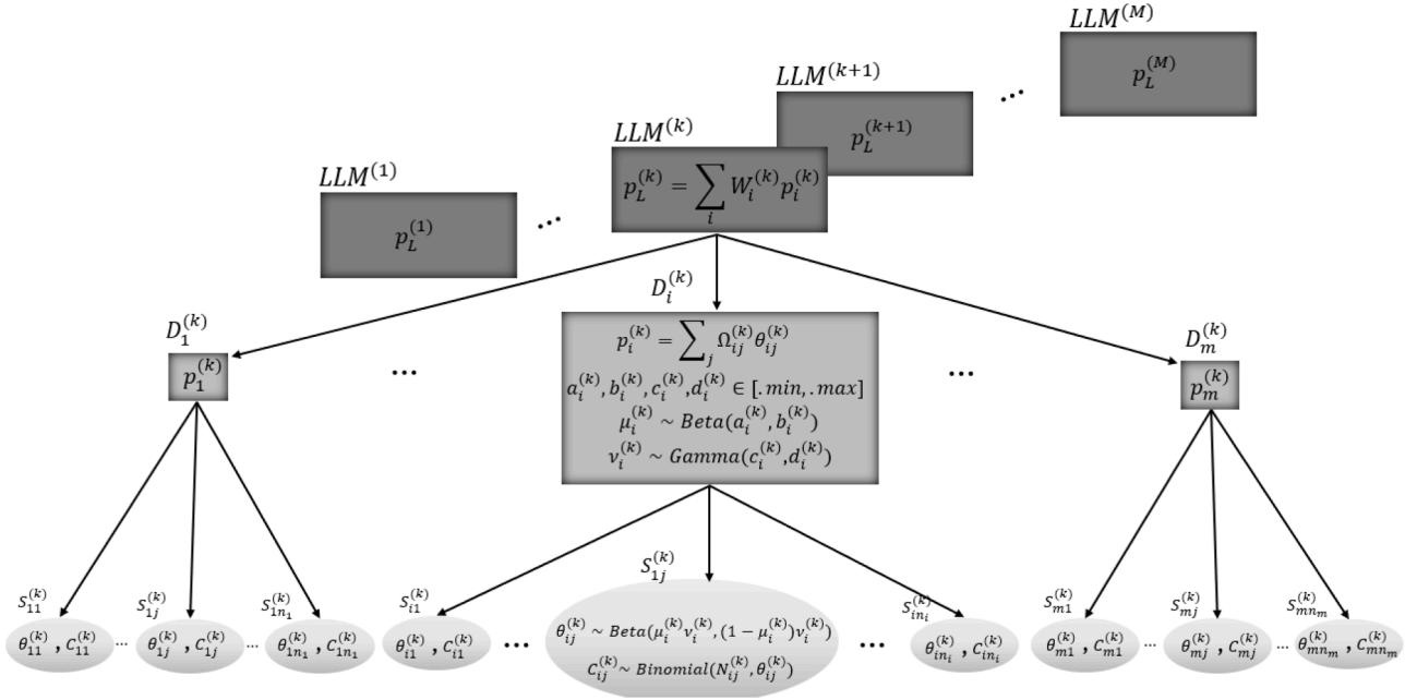
Fig. 2. Hierarchical structure with independent domains and dependent subdomains. For readability, parameters and priors are shown only for one subdomain S_{ij} and its parent domain D_i under a representative LLM_i ; the remaining subdomains, domains ( i = 1, \dots, m ), and LLMs ( k = 1, \dots, M ) are identical, differing only in their indices. Rectangles indicate independent components, while ovals indicate dependent components within the hierarchy.
