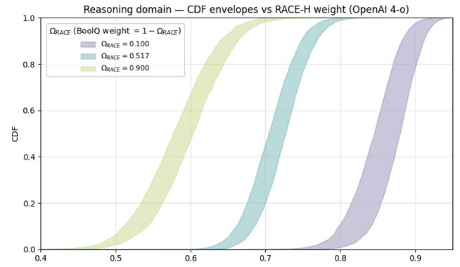
(b) Posterior CDF envelopes of non-failure probability for the Reasoning domain ( D_2 ) under alternative operational weights on RACE-H, for OpenAI 4-o.
