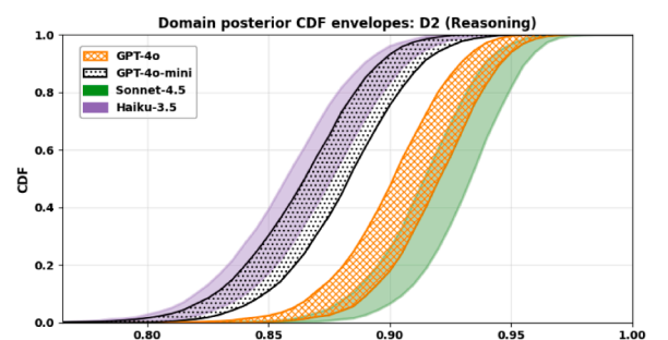
(b) Posterior CDF envelopes of non-failure probability p_2 = \sum_j \Omega_{2j} \theta_{2j} for Dom 2 (reasoning) across four models, with subdomain-level operational weights (0.483, 0.517) .
