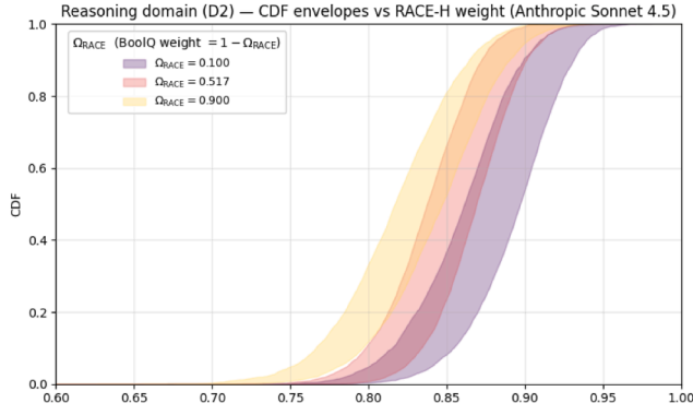
(a) Posterior CDF envelopes of non-failure probability for the Reasoning domain ( D_2 ) under alternative operational weights on RACE-H, for Anthropic Sonnet 4.5.
