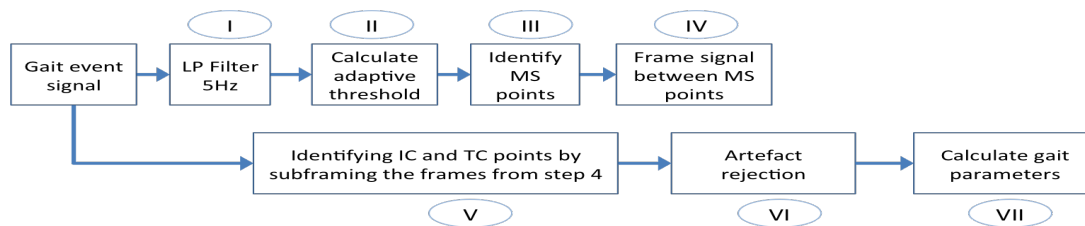
Figure 3: Framing algorithm.
