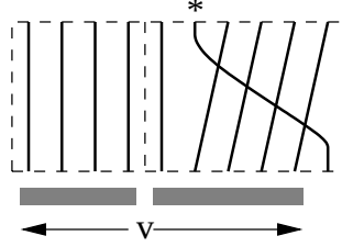
Fig. 9. Realising the element (v, j) as a diagram.
