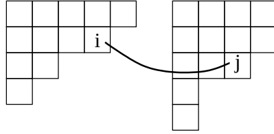
Fig. 11. A graphical representation of the arc ij in w_0
