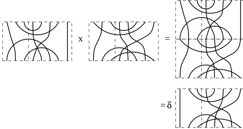
Fig. 2. The product of two basis elements in B_{3,5}(\delta) .
