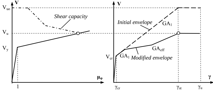
Fig. 4 (a) Flexural primary curve in terms of member shear force and curvature ductility demand of the critical cross section. (b) Shear ( V - \gamma ) primary curve before and after modelling shear-flexure interaction
