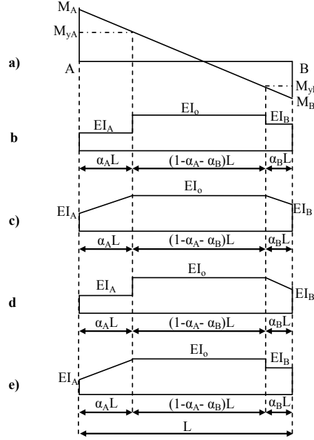
Fig. 3 Element. (a) Bending moment diagram. (b) Stiffness distribution when ends A and B are in the loading state. (c) Stiffness distribution when ends A and B are in the unloading or reloading state. (d) Stiffness distribution when end A is in the loading and end B is in the unloading or reloading state. (e) Stiffness distribution when end A is in the unloading or reloading state and end B is in the loading state
