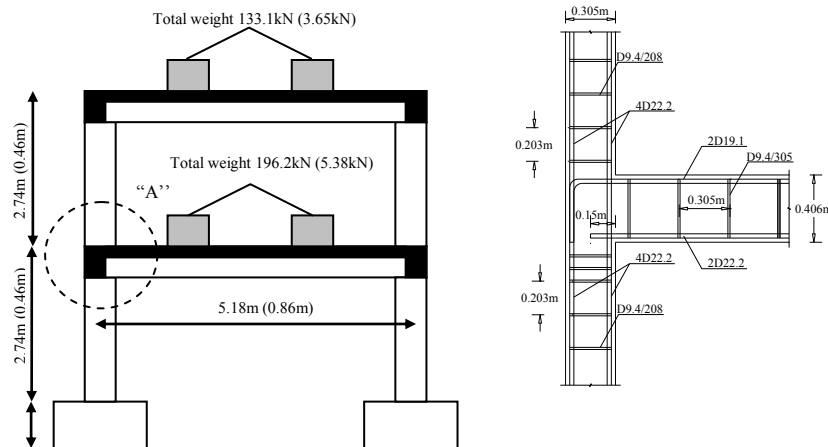
Fig. 18 (a) El-Attar et al. (1997) frame specimen configuration (values outside and inside parentheses correspond to model and experimental values, respectively)
