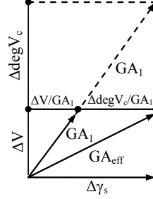
Fig. 6 Determination of effective shear stiffness GA_{eff}
