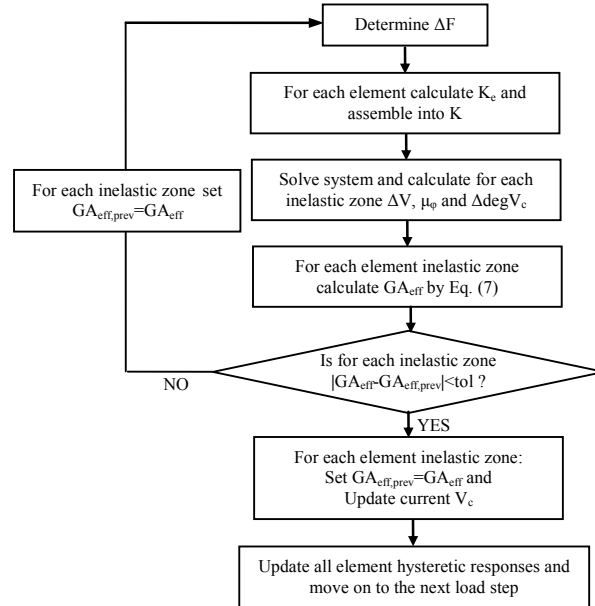
Fig. 12 Shear-flexure interaction implementation algorithm
