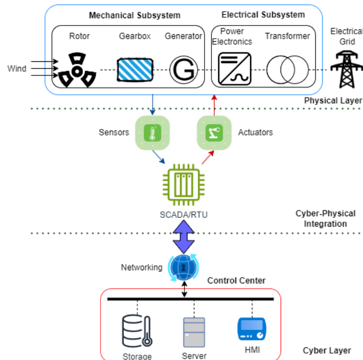
Figure 2. Wind power plant as a CPS [19].
