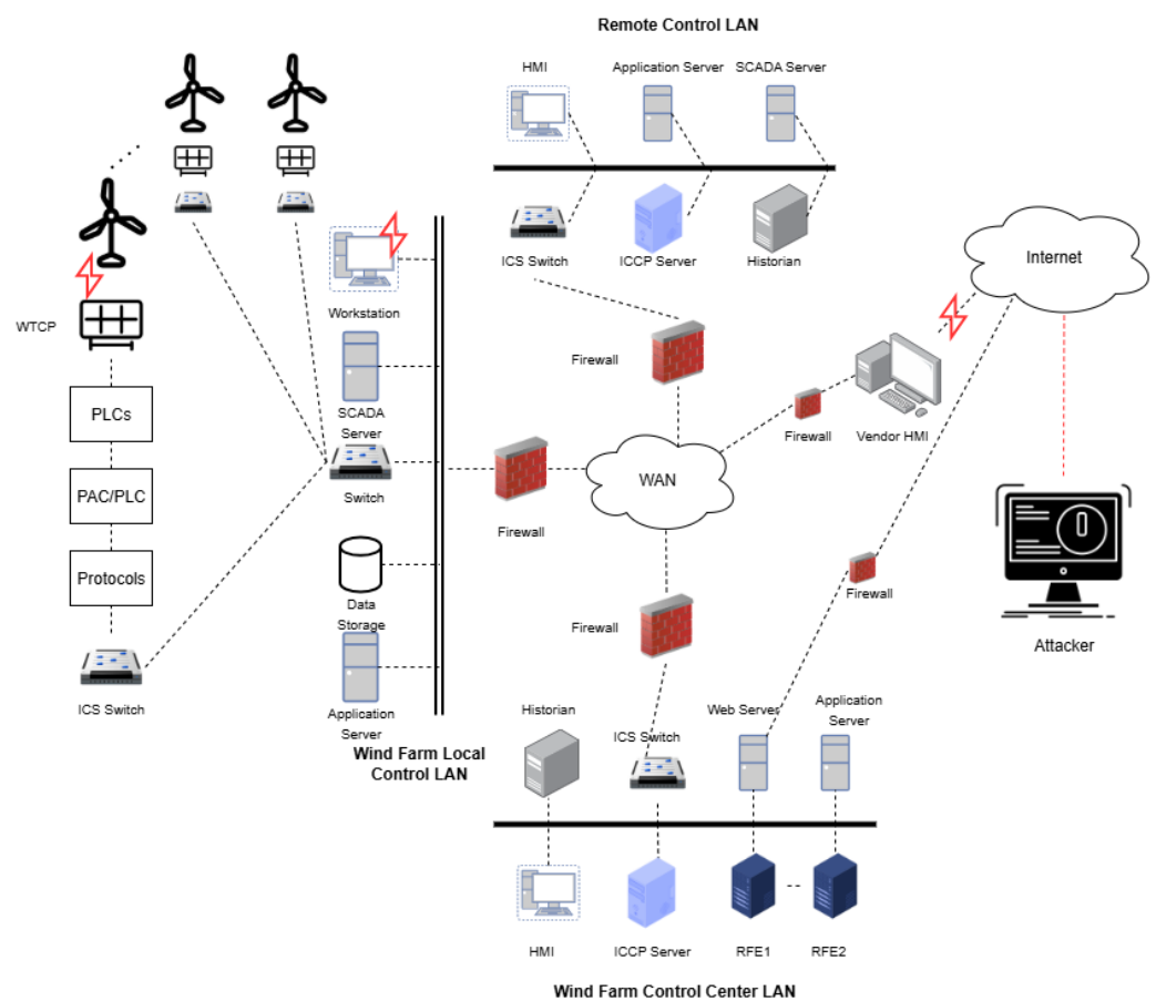
Figure 3. The SCADA network in a wind farm [20].
