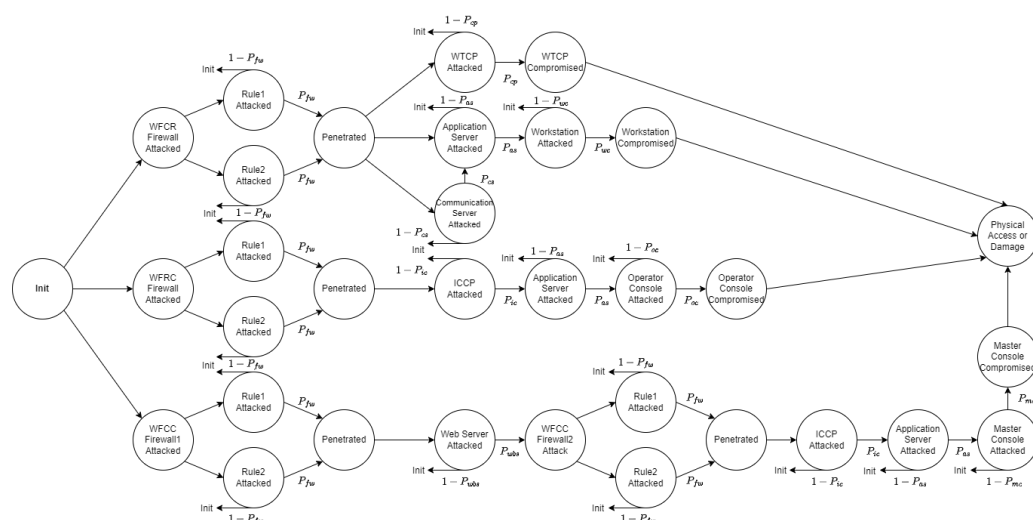
Figure A1. MDP-based attack model for wind power plants.
