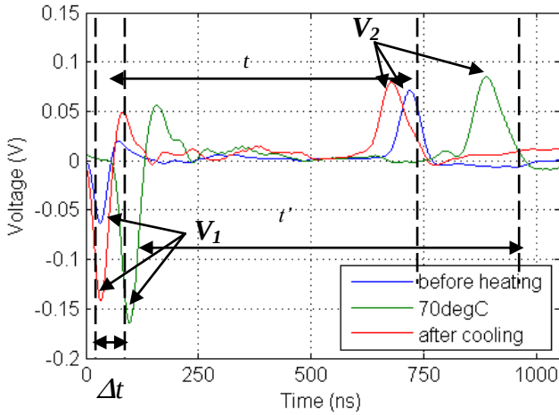
Fig. 4. Averaged raw output of the flat electrode PEA system with +8kVDC bias voltage and a clamping force of 250N applied on a 30mm cable clamp.
