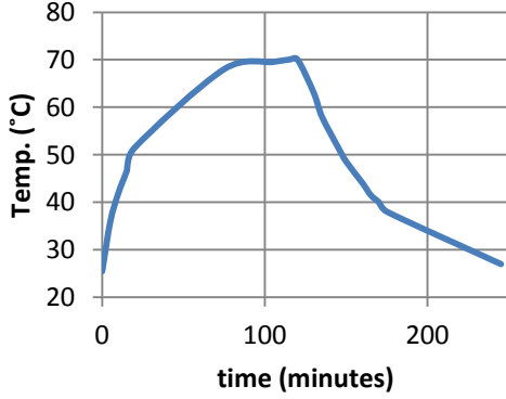
Fig. 3. Temperature of the PEA cell during heating and cooling processes of the thermal cycle.
