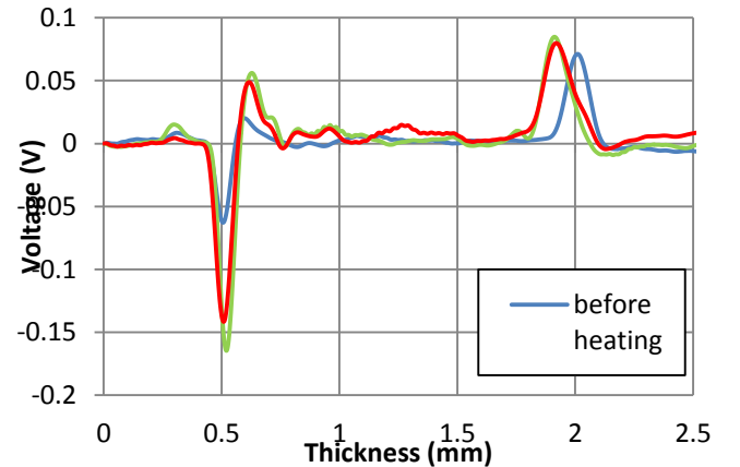
Fig. 5. Averaged raw data rescaled to correct for acoustic velocity difference at 25 °C and 70 °C and with time axis converted to distance.
