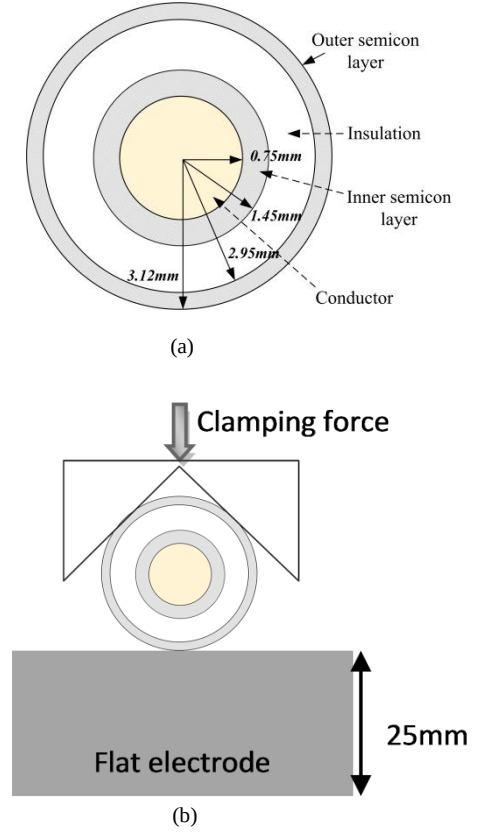
Fig. 2. (a) Structure and dimensions of mini-cables. (b) Schematic diagram of the PEA cell with the flat electrode.
