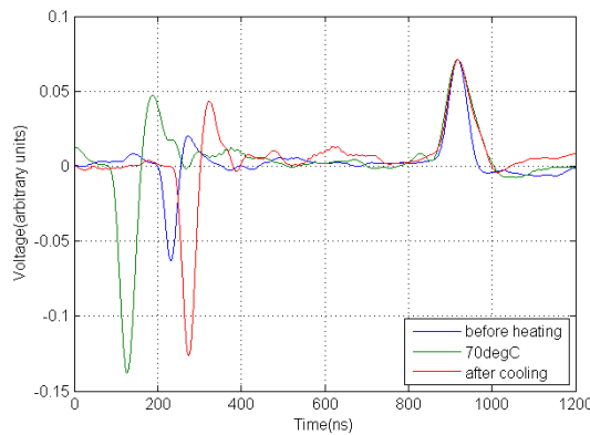
Fig. 7. Averaged raw output signal after normalisation of the amplitudes of the second peak, V_2 . Time has been shifted to align peak V_2 for the three sets of data.
