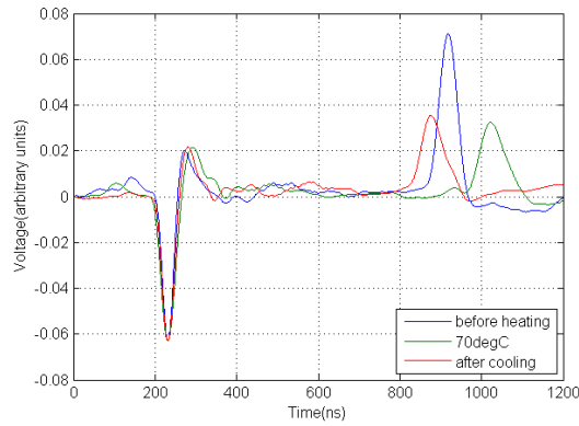
Fig. 6. Averaged raw output signal after normalisation of the amplitudes of the first peak, V_1 . Time has been shifted to align peak V_1 for the three sets of data.
