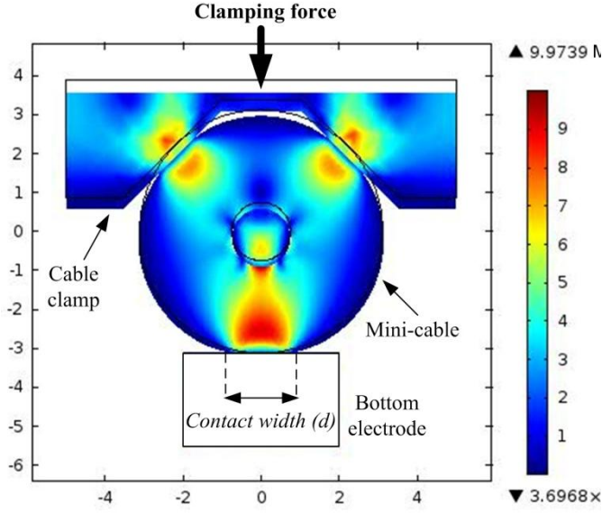
Fig.1 Surface plot of the von Mises stress [10] on the cross-section of mini-cable when applying 470N clamping force (semicon layer and insulation are included in the same domain due to their similar mechanical properties). [9]
